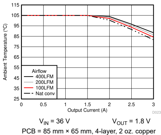
Figure 6-23. Safe Operating Area
