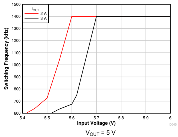
7-10. Frequency Foldback
