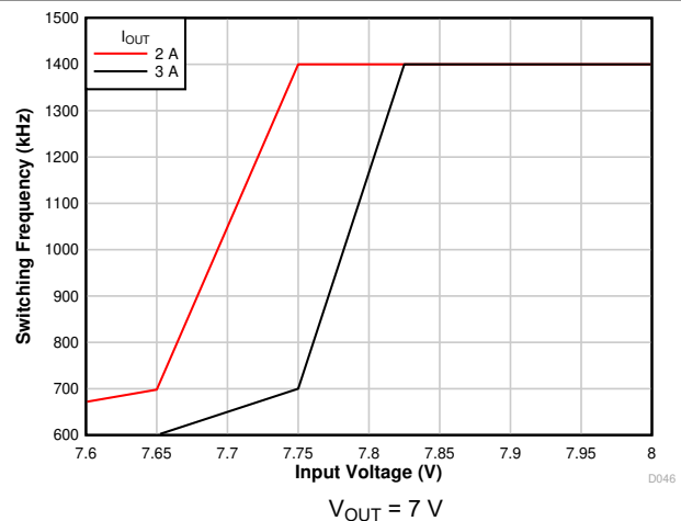
7-12. Frequency Foldback
