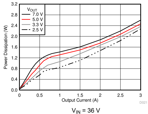
Figure 6-21. Power Dissipation versus Output Current
