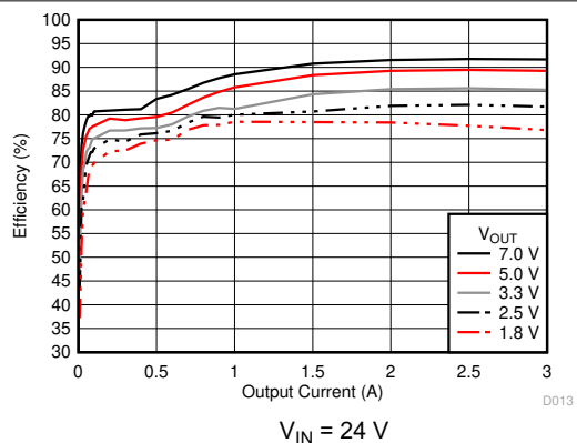
Figure 6-13. Efficiency versus Output Current
