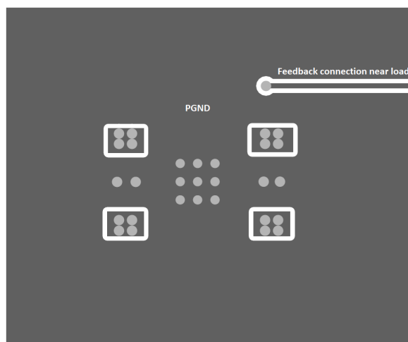
Figure 10-3. Typical PGND Layer
