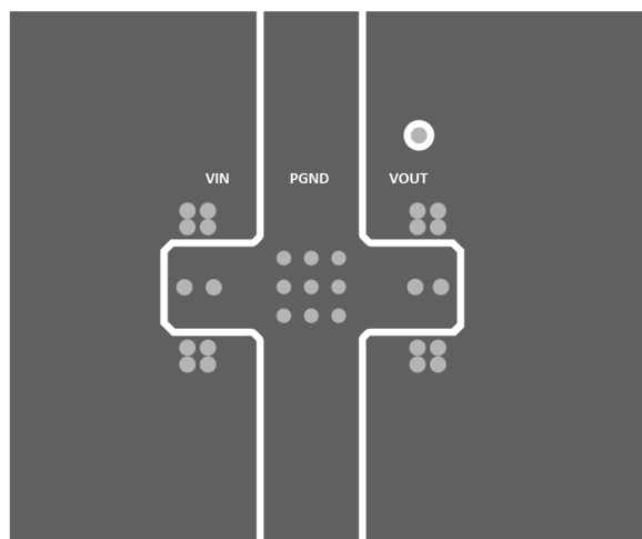
Figure 10-2. Typical Layer-2 Layout
