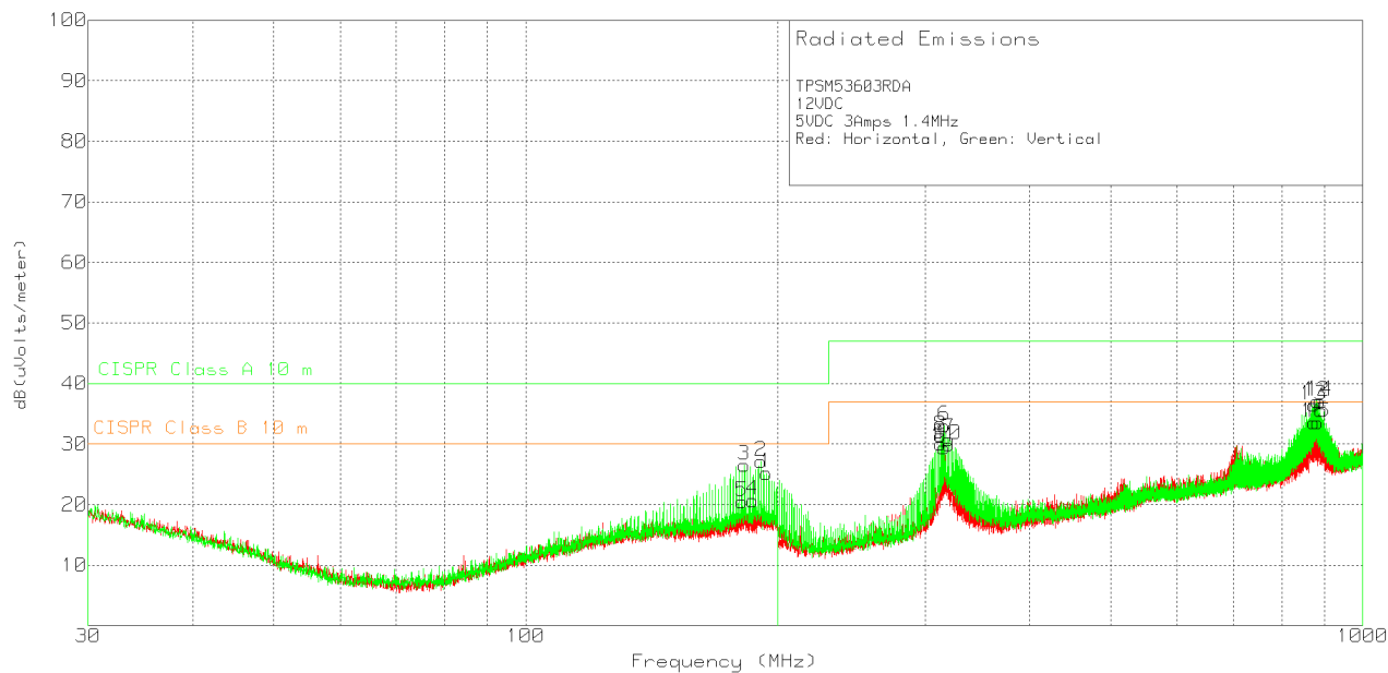
✎ 10-6. Radiated Emissions 12-V Input, 5-V Output, 3-A Load
