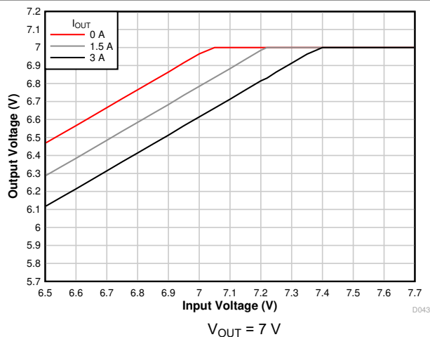
7-11. Voltage Dropout
