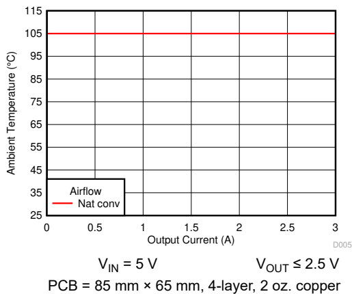
6-5. Safe Operating Area
