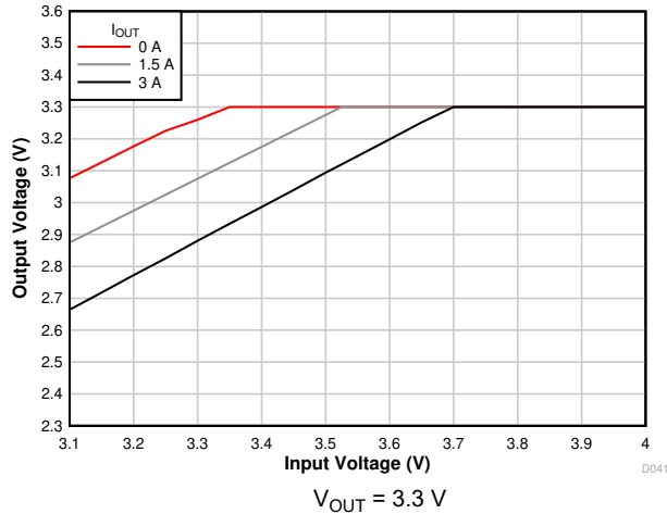
7-7. Voltage Dropout
