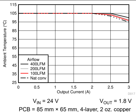
Figure 6-17. Safe Operating Area
