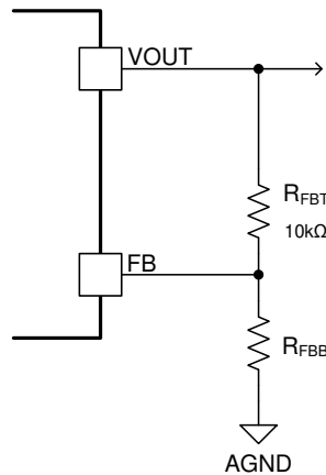
図 7-1. Setting the Output Voltage
