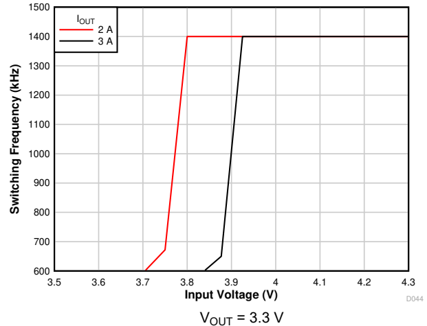
7-8. Frequency Foldback
