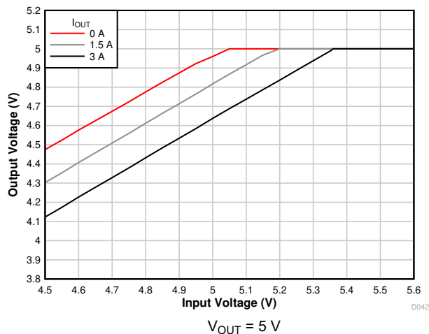
7-9. Voltage Dropout
