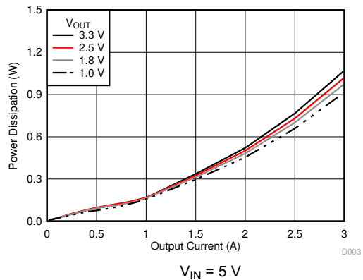
6-3. Power Dissipation versus Output Current
