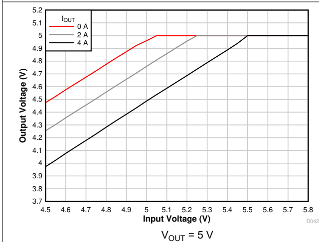
7-9. Voltage Dropout
