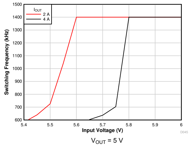
7-10. Frequency Foldback
