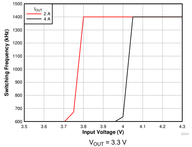
7-8. Frequency Foldback
