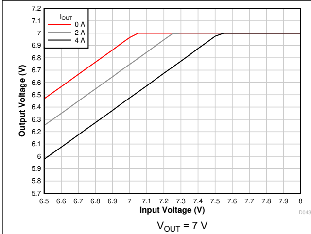
7-11. Voltage Dropout
