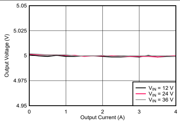
9-3. Load Regulation
