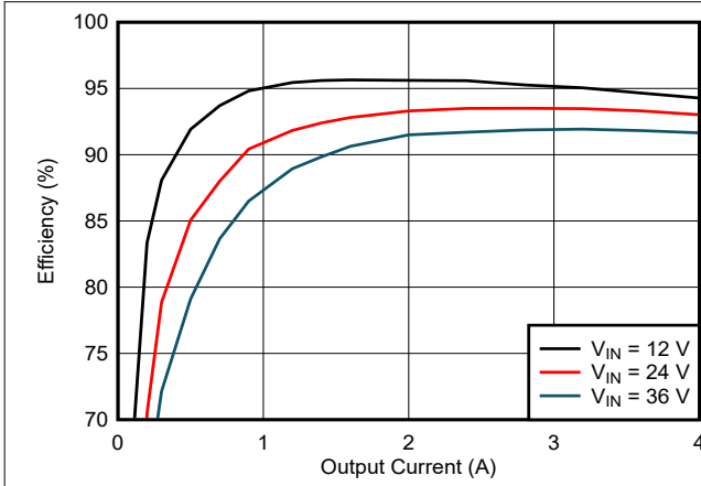
9-2. Efficiency
