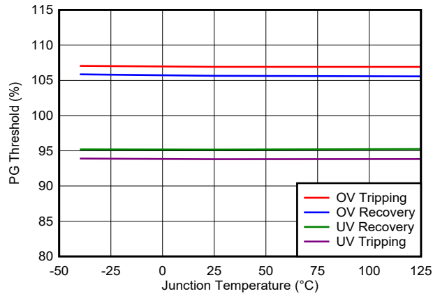
7-7. Power Good (PG) Thresholds
