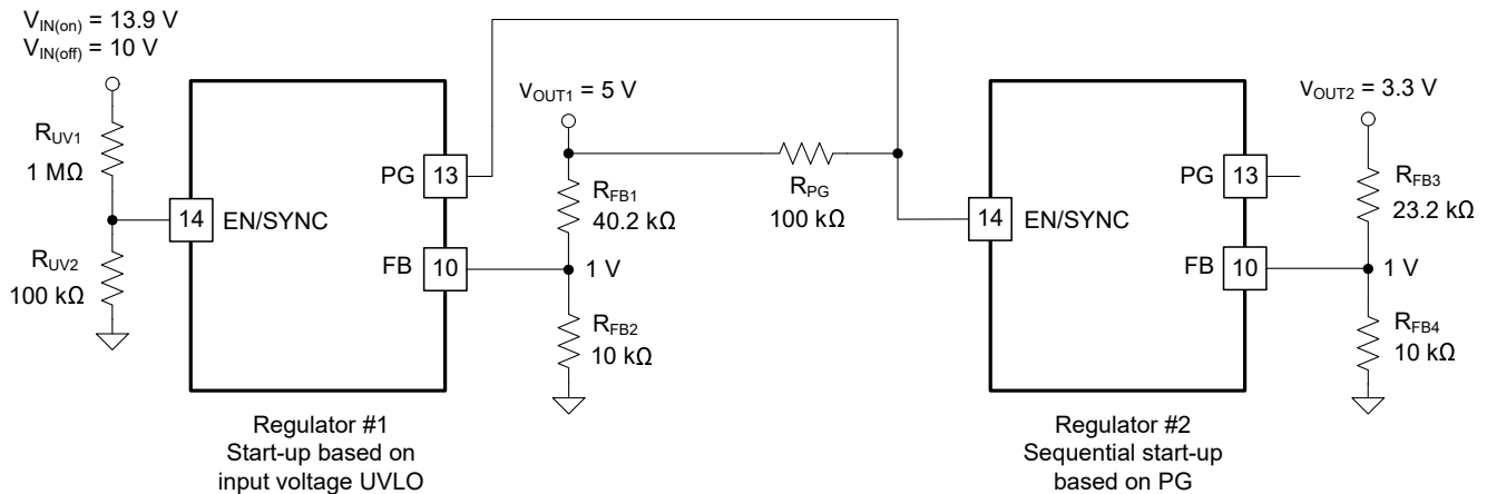
Figure 8-3. TPSM63604 Sequencing Implementation Using PG and EN/SYNC
