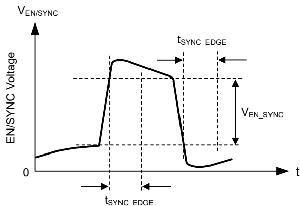
图 8-2. Typical SYNC Waveform
