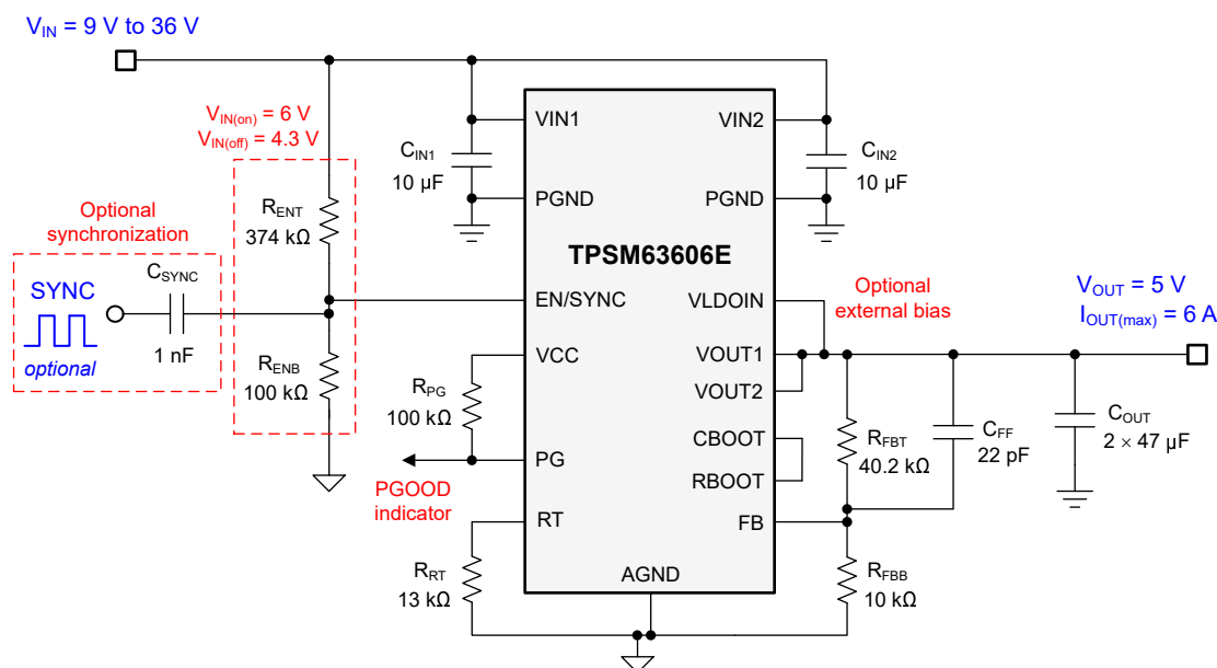
9-1. Circuit Schematic
