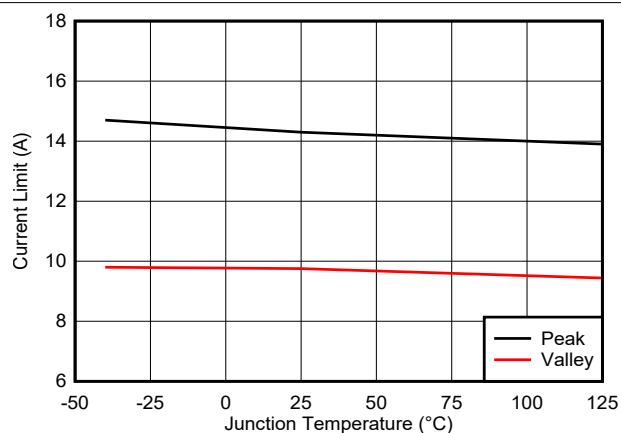
図 7-4. High-Side (Peak) and Low-Side (Valley) Current Limits TPSM63610
