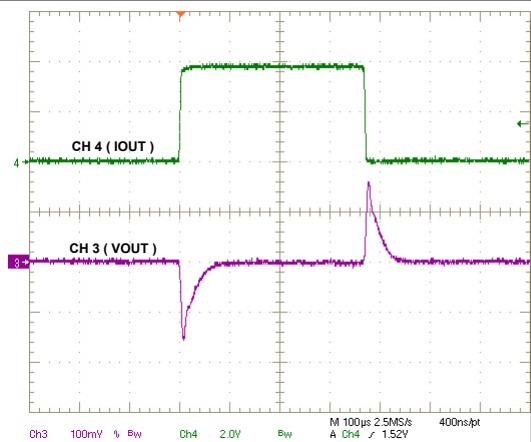
図 9-8. Load Transient, 0 A to 4 A, 1 A/ \mu s
