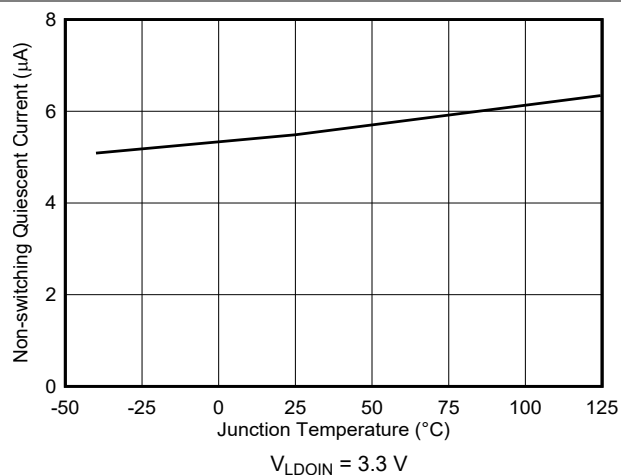
図 7-2. Non-Switching Input Supply Current
