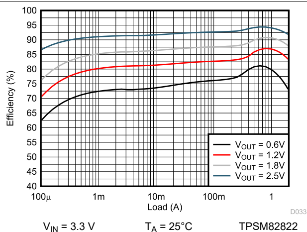
9-57. Efficiency
