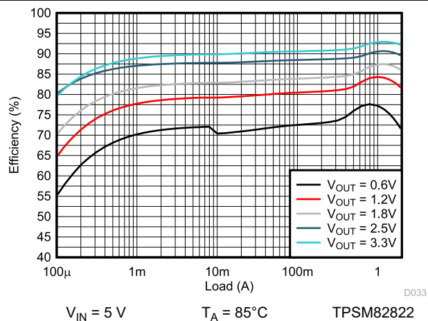
9-54. Efficiency
