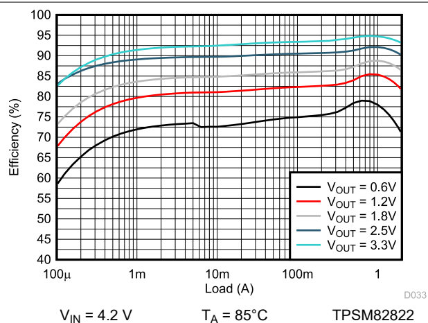
9-56. Efficiency
