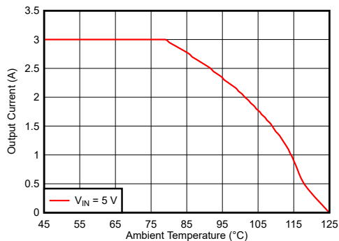
FIG 9-122. Safe Operating Area
