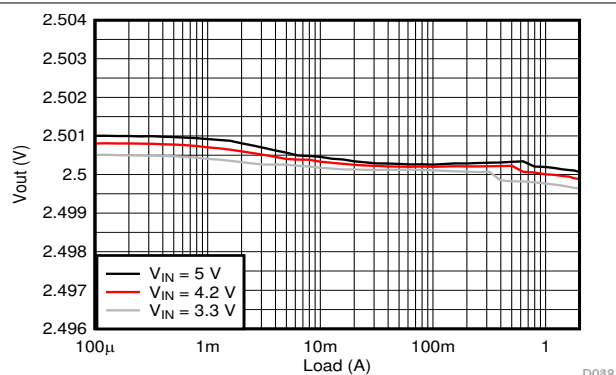
9-67. Load Regulation
