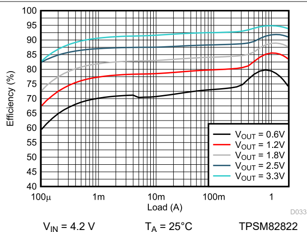
9-55. Efficiency
