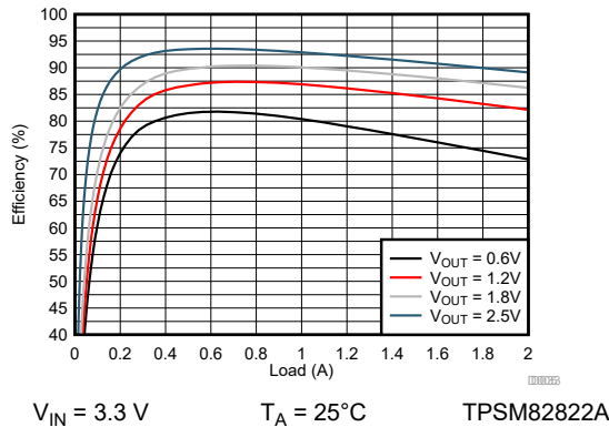
Figure 9-90. Efficiency
