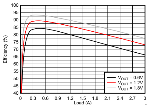
图 9-143. Efficiency
