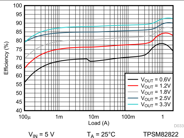
9-53. Efficiency
