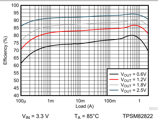
9-58. Efficiency
