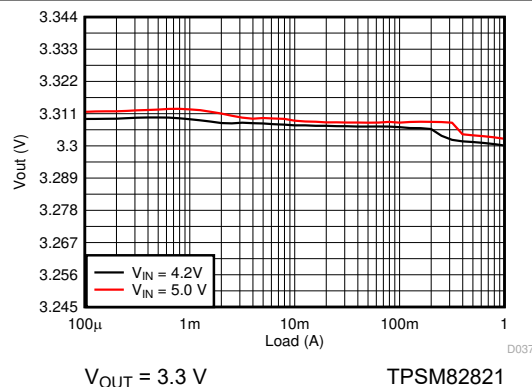
9-20. Load Regulation
