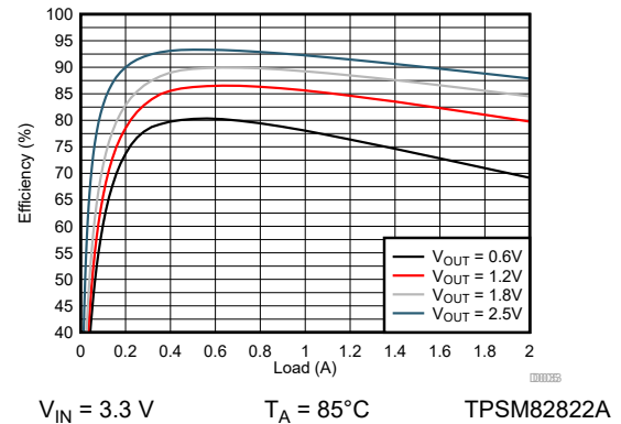
Figure 9-91. Efficiency
