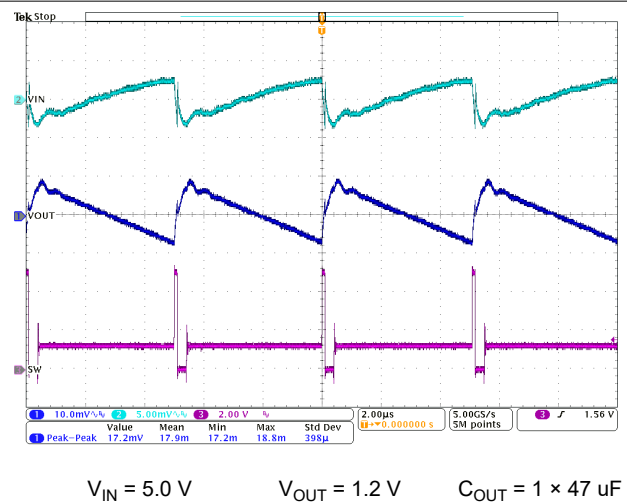
8-29. PSM Operation I_{OUT} = 0.1\text{ A}
