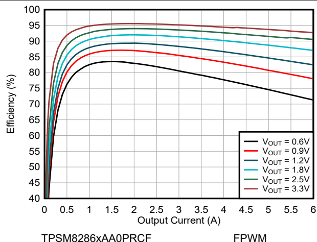
図 8-3. Efficiency V_{IN} = 5.0\text{ V} and T_A = 85^\circ\text{C}
