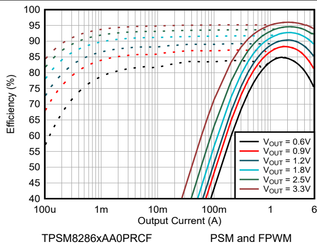
図 8-2. Efficiency V_{IN} = 5.0\text{ V} and T_A = 25^\circ\text{C}
