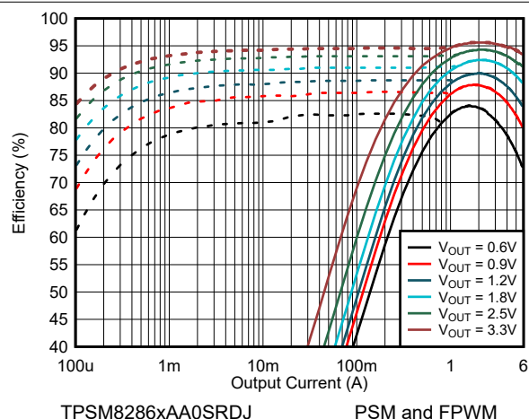
図 8-8. Efficiency V_{IN} = 5.0\text{ V} and T_A = 25^\circ\text{C}
