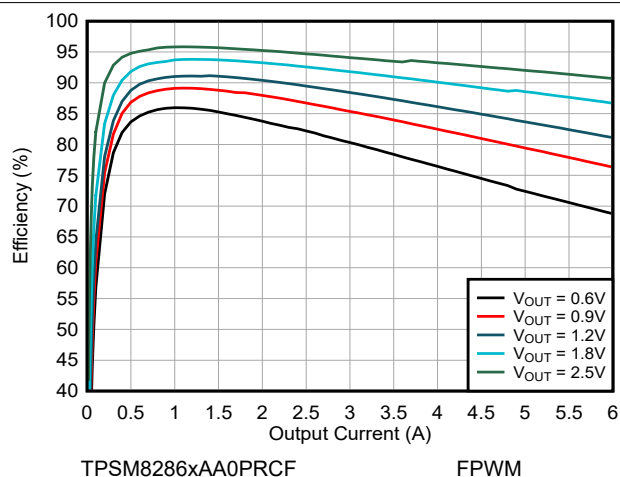
図 8-5. Efficiency V_{IN} = 3.3\text{ V} and T_A = 85^\circ\text{C}
