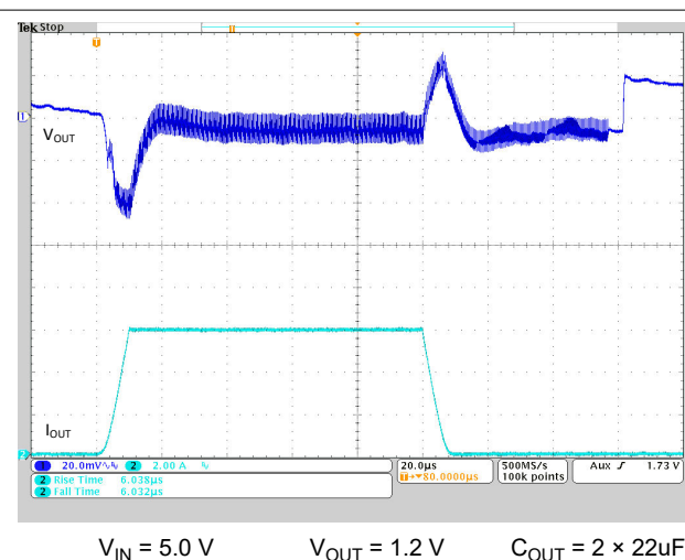
図 8-33. Load Transient PSM I_{OUT} = 0 \text{ A} \rightarrow 6 \text{ A}
