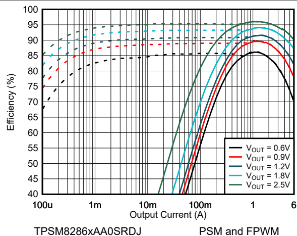
図 8-10. Efficiency V_{IN} = 3.3\text{ V} and T_A = 25^\circ\text{C}
