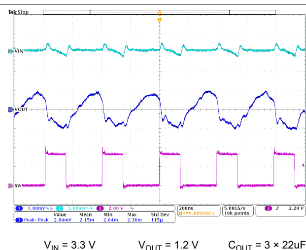
図 8-31. FPWM Operation I_{OUT} = 0.1 \text{ A}
