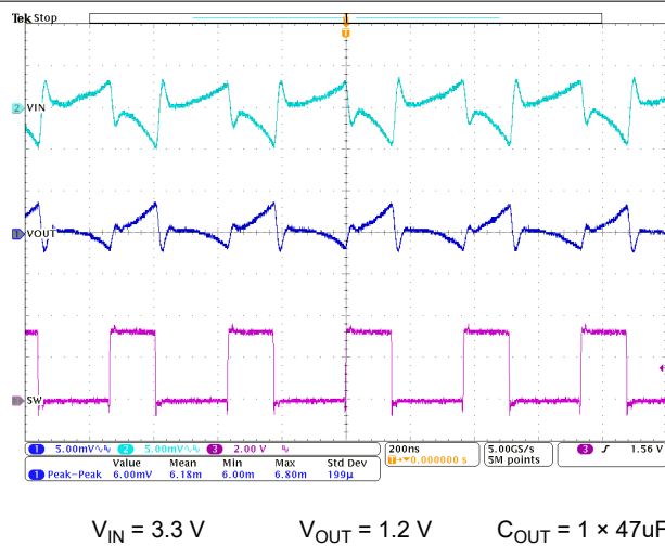
8-28. FPWM Operation I_{OUT} = 3\text{ A}
