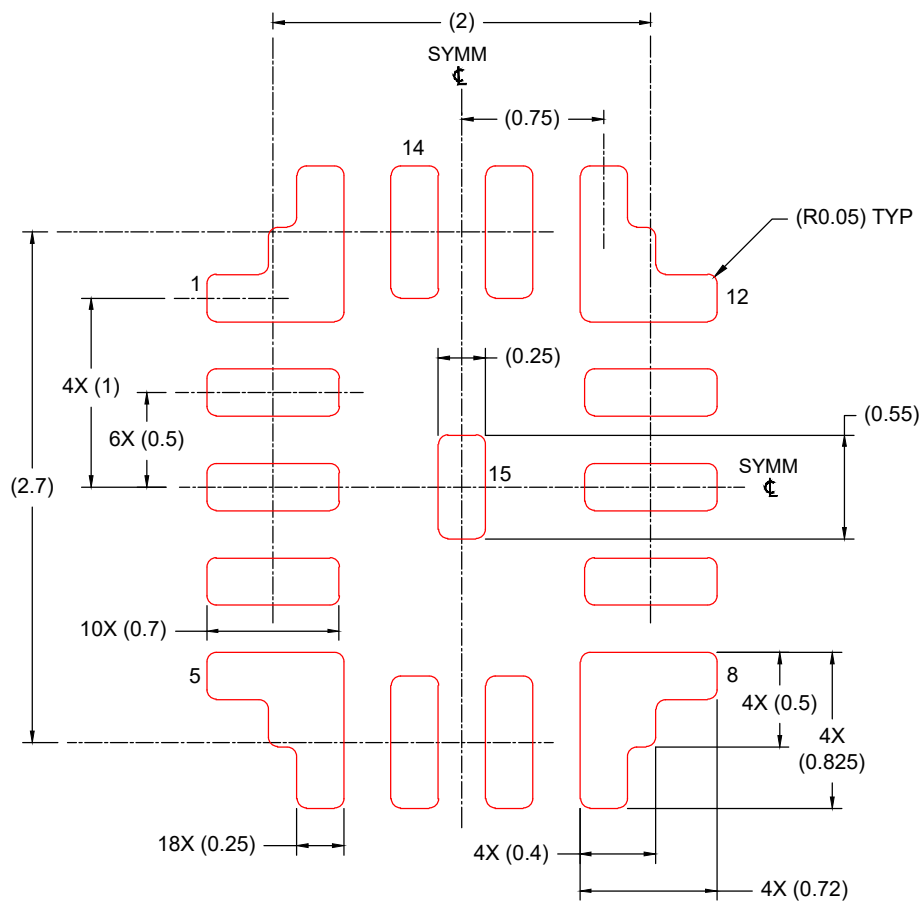
SOLDER PASTE EXAMPLE BASED ON 0.1 mm THICK STENCIL SCALE: 25X
