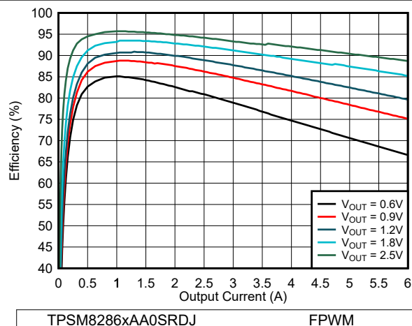
図 8-11. Efficiency V_{IN} = 3.3\text{ V} and T_A = 85^\circ\text{C}
