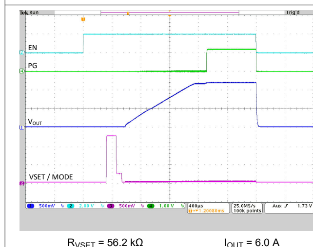
図 8-34. Start-Up into Full Load
