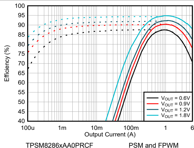
図 8-6. Efficiency V_{IN} = 2.8\text{ V} and T_A = 25^\circ\text{C}
