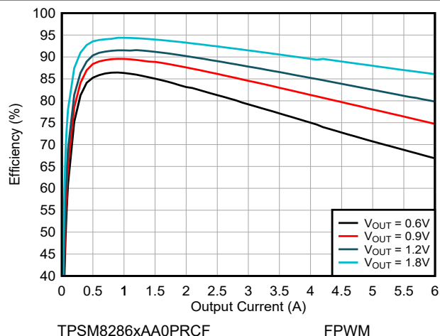
図 8-7. Efficiency V_{IN} = 2.8\text{ V} and T_A = 85^\circ\text{C}
