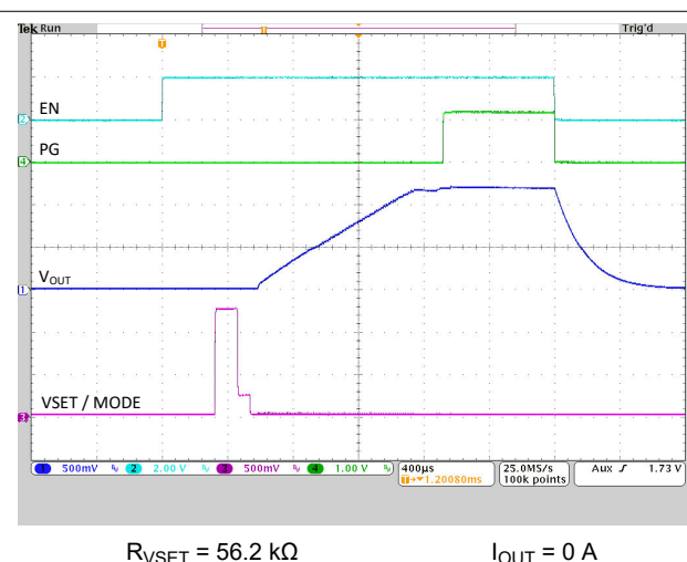
図 8-35. Start-Up with No Load
