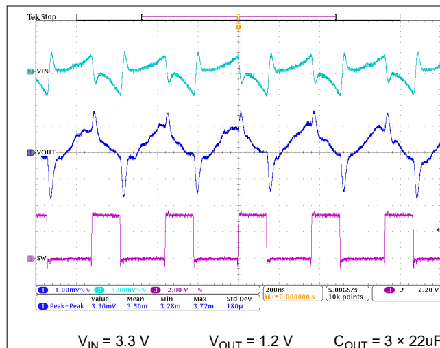
図 8-30. FPWM Operation I_{OUT} = 3 \text{ A}
