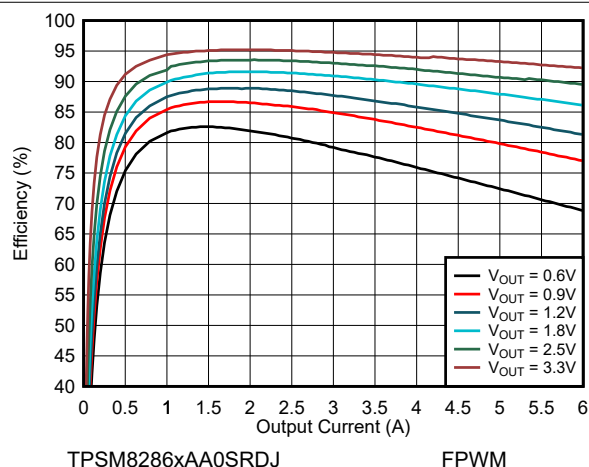
図 8-9. Efficiency V_{IN} = 5.0\text{ V} and T_A = 85^\circ\text{C}
