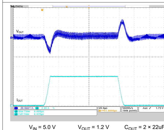
図 8-32. Load Transient FPWM I_{OUT} = 0 \text{ A} \rightarrow 6 \text{ A}
