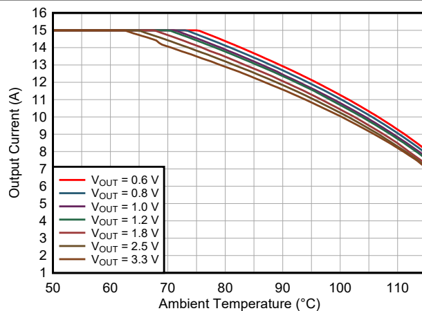
図 9-49. Safe Operating Area TPSM8287A15BBH V_{IN} = 5.0\text{ V}
