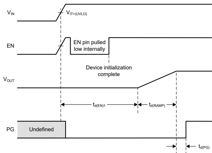
Figure 7-11. Start-Up Timing When EN is Pulled Up to V IN
