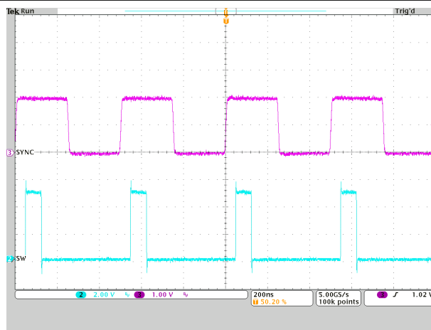
図 9-31. Synchronization to an External Clock
