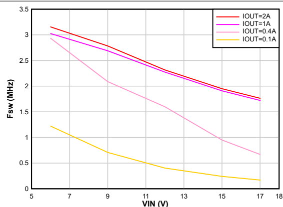
8-19. Switching Frequency vs Input Voltage V OUT = 1.8 V
