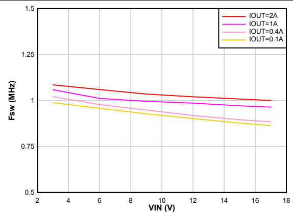
8-18. Switching Frequency vs Input Voltage V OUT = 1.8 V
