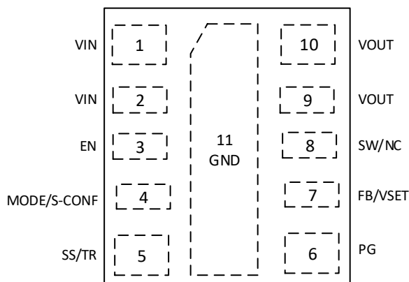
図 5-1. 11-Pin SIS MicroSiP™ Package (Top View, Device Pins Face Down)
