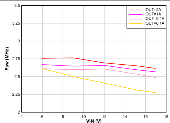
8-20. Switching Frequency vs Input Voltage V OUT = 1.2 V
