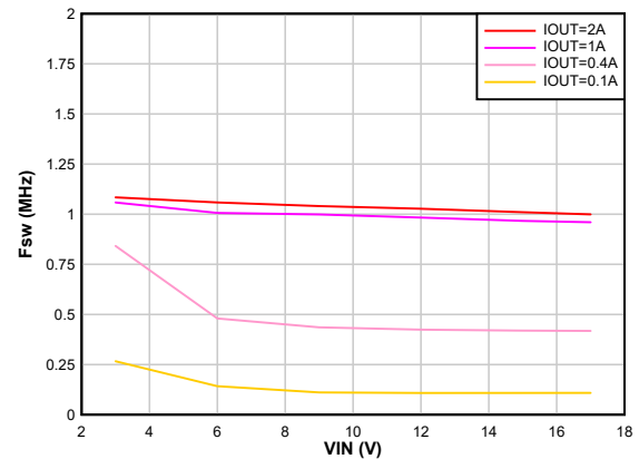
8-18. Switching Frequency vs Input Voltage V OUT = 1.8 V
