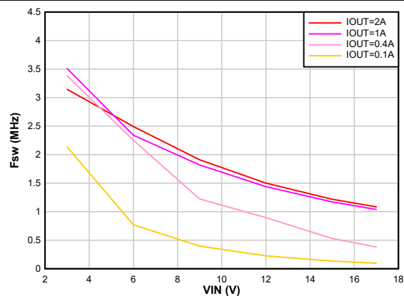
8-17. Switching Frequency vs Input Voltage V OUT = 1.2 V
