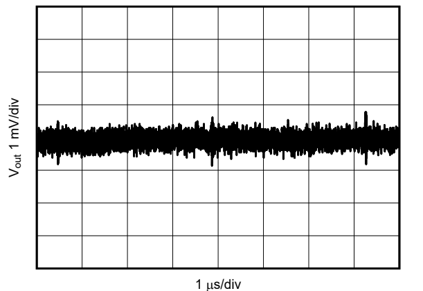
图 6-19. V_{OUT} Ripple After the Second L-C Filter
