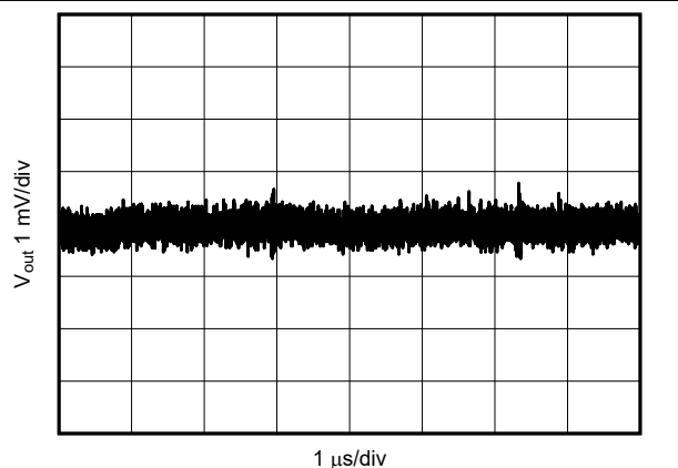
图 6-23. V_{OUT} Ripple After the Second L-C Filter
