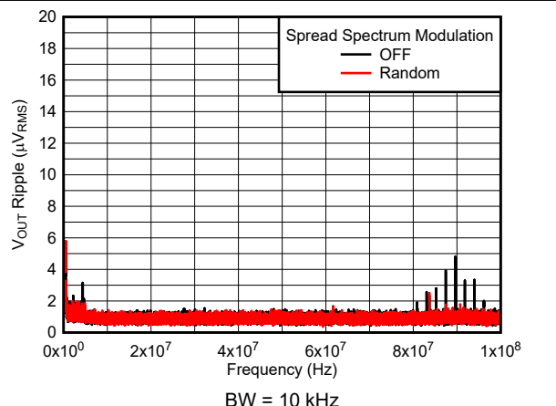
图 6-22. V_{OUT} Ripple FFT After the First L-C Filter
