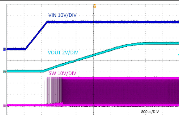
図 7-10. Start-Up Relative to V_{IN} , I_{OUT} = 3A
