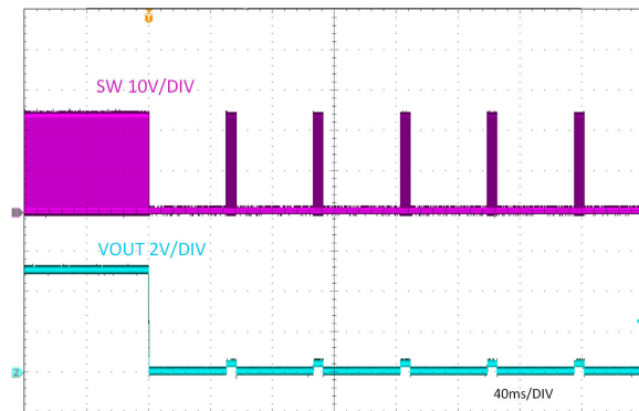
7-15. V OUT Hard Short Protection
