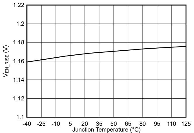
図 5-4. Enable Threshold vs Junction Temperature
