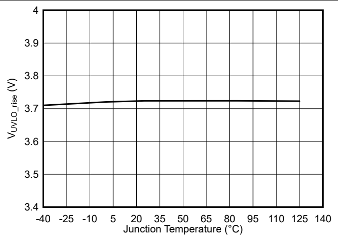
図 5-6. V_{IN} UVLO Rising Threshold vs Junction Temperature
