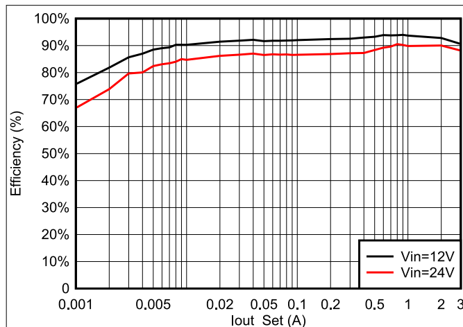
図 7-2. Efficiency (PFM)
