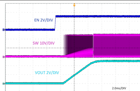
図 7-11. Start-Up Through EN, I_{OUT} = 3A
