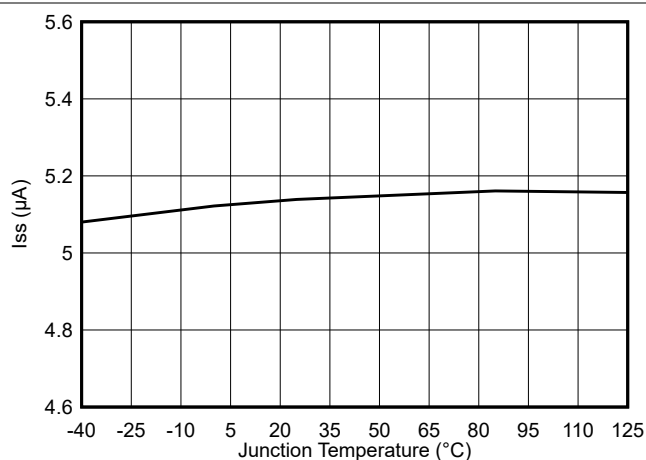
図 5-13. Soft-Start Charge Current vs Junction Temperature
