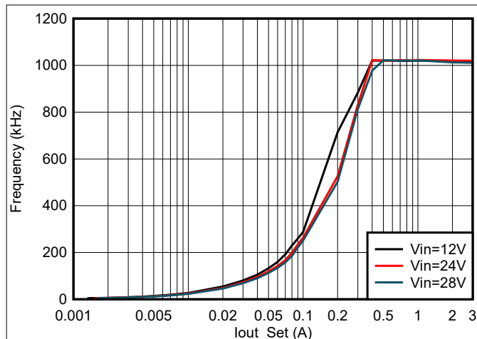
図 7-8. Switching Frequency vs Load Current
