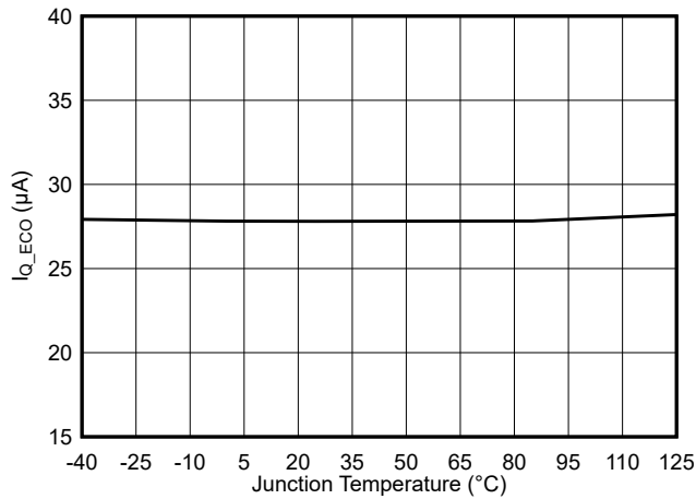
図 5-1. TPSM84338 Quiescent Current (PFM) vs Junction Temperature
