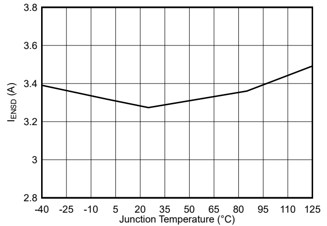
図 5-2. TPSM84338 Shutdown Current vs Junction Temperature
