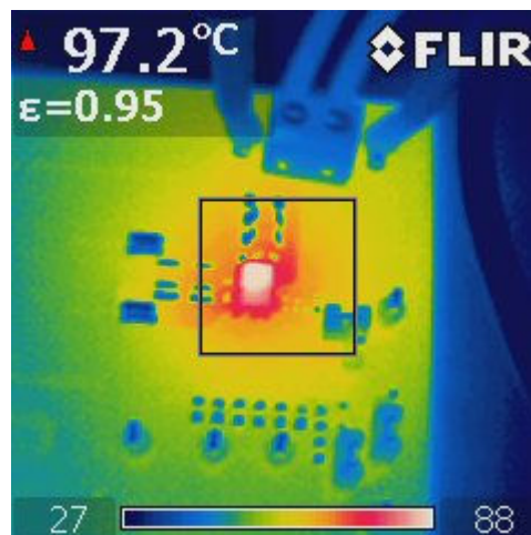
図 7-9. Case Temperature, V_{IN} = 24V , I_{OUT} = 3A , f_{sw} = 1000kHz
