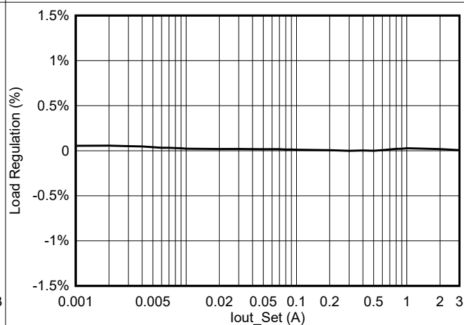
図 5-16. TPSM84338 Load Regulation (FCCM), V_{IN} = 24\text{V} , V_{OUT} = 12\text{V} , f_{SW} = 2200\text{kHz}
