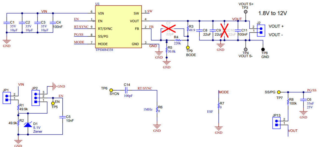
7-1. TPSM84338 5V Output, 3A Reference Design
