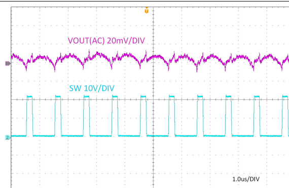
図 7-13. Steady State, I_{OUT} = 3A
