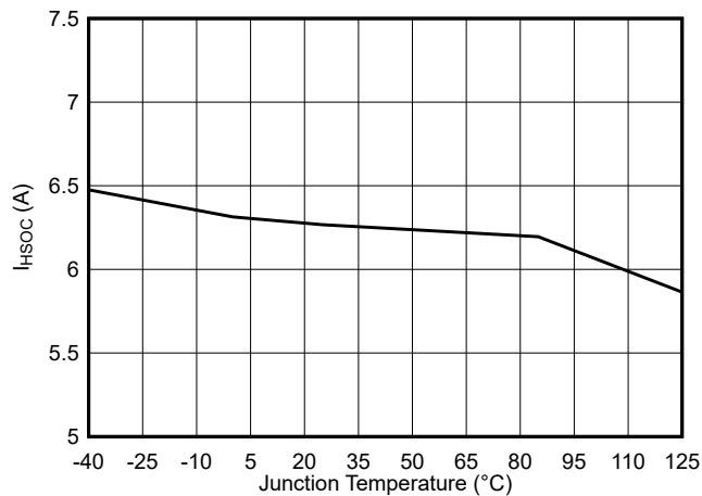
■ 5-9. TPSM84338 High-Side Current Limit vs Junction Temperature
