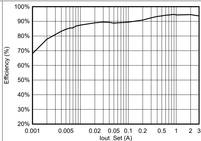
図 5-14. TPSM84338 Efficiency (PFM), V_{IN} = 24\text{V} , V_{OUT} = 12\text{V} , f_{SW} = 2200\text{kHz}
