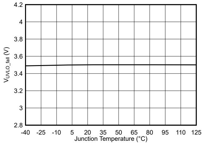
■ 5-7. V_{IN} UVLO Falling Threshold vs Junction Temperature
