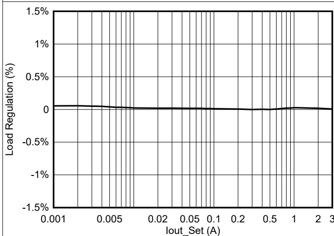
図 5-15. TPSM84338 Load Regulation (PFM), V_{IN} = 24\text{V} , V_{OUT} = 12\text{V} , f_{SW} = 2200\text{kHz}
