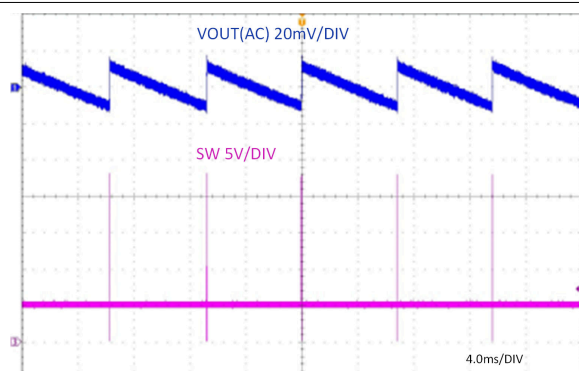
図 7-12. Steady State, I_{OUT} = 0A
