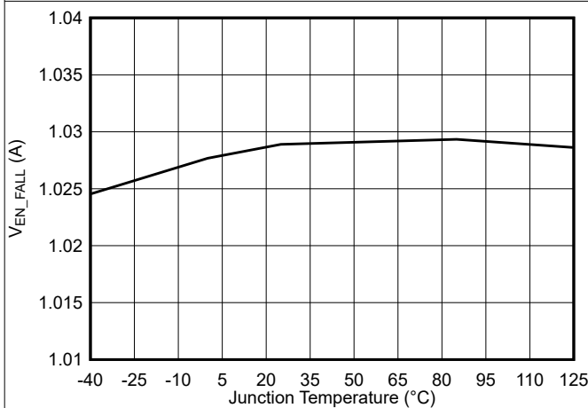
図 5-5. Disable Threshold vs Junction Temperature
