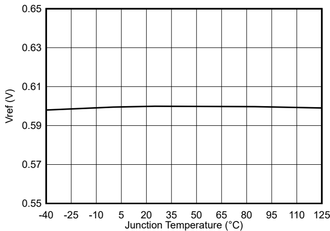
図 5-3. Feedback Voltage vs Junction Temperature
