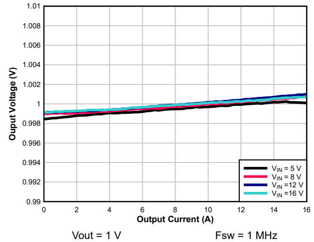
图 8-5. Load Regulation
