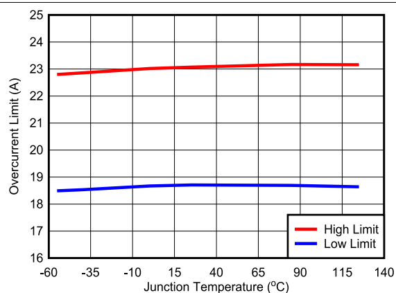
Figure 6-3. Overcurrent Limit
