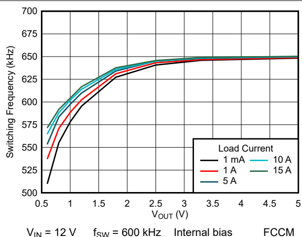
图 8-24. Switching Frequency
