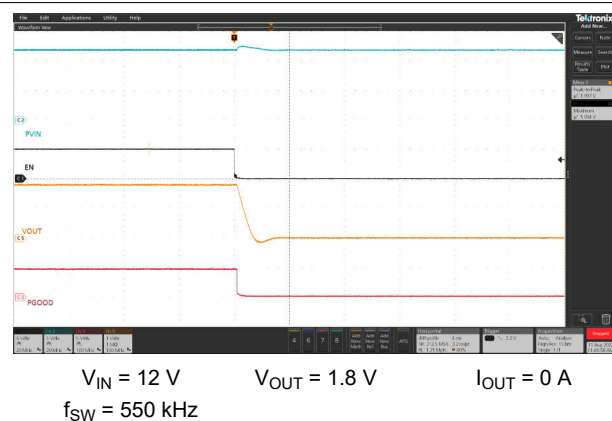
8-22. Shutdown from CNTL
