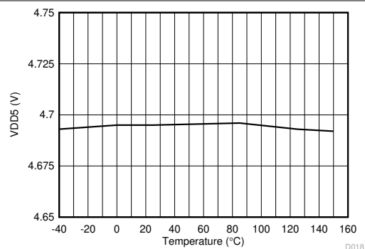
図 6-12. VDD5 Voltage vs Junction Temperature
