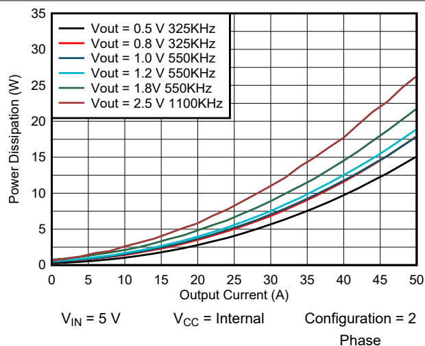
Figure 6-6. TPSM8D6B24 Efficiency vs Output Current
