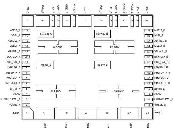
図 5-2. 59-Pin QFM-MOW Package (Bottom View)
