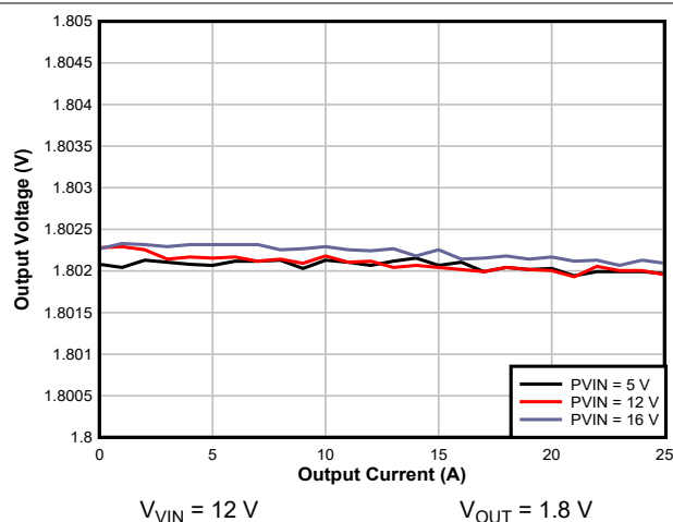
8-3. Load Regulation
