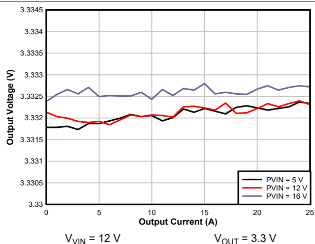
8-4. Load Regulation
