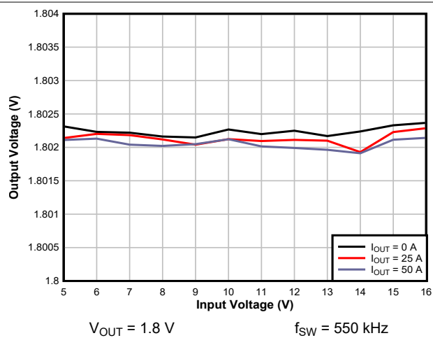
8-20. Line Regulation
