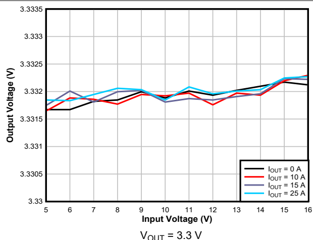
8-6. Line Regulation
