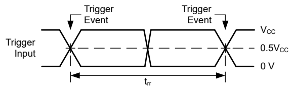
Figure 6-4. Voltage Waveforms, Retriquer Time
