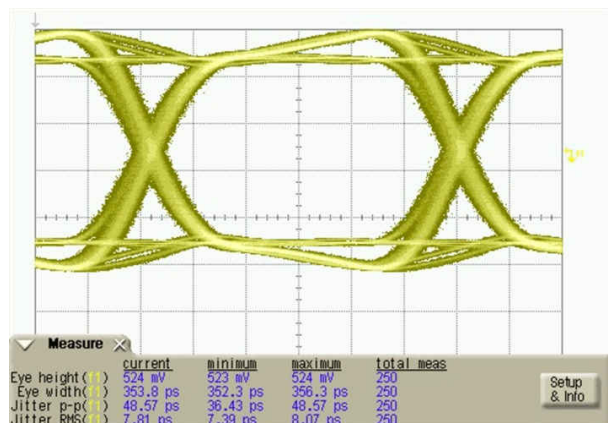
8-1. TSB82AF15-EP Eye Diagram
