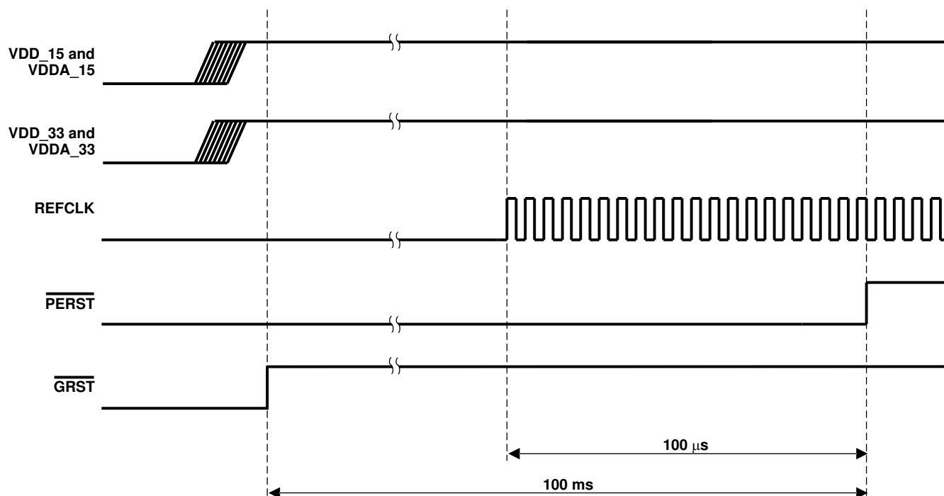
FIG 10-2. Power-Up Sequence
