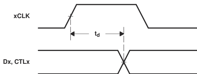
9-2. Dx and CTLx Output Delay Relative to xCLK Waveforms
