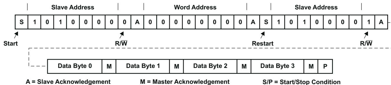
10-11. Serial-Bus Protocol Multibyte Read
