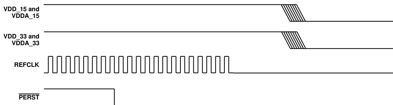
FIG 10-3. Power-Down Sequence
