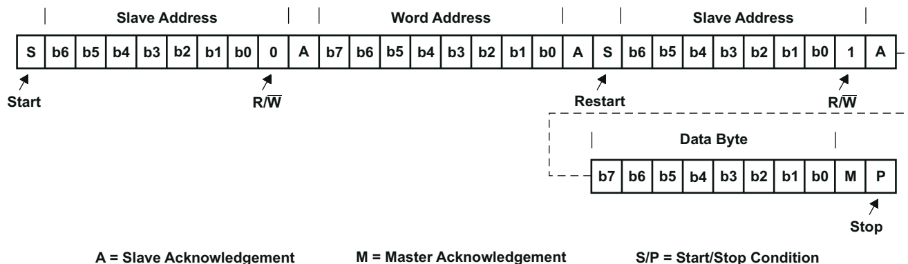
10-10. Serial-Bus Protocol Byte Read
