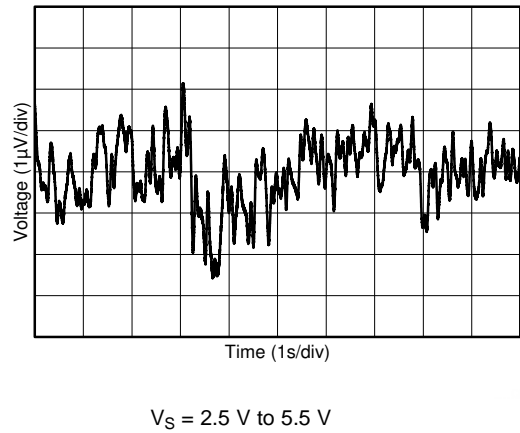
14. 0.1-Hz to 10-Hz Input Voltage Noise
