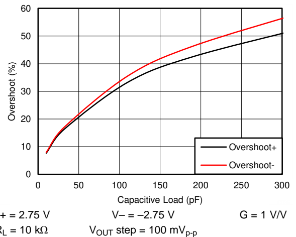
22. Small-Signal Overshoot vs Load Capacitance
