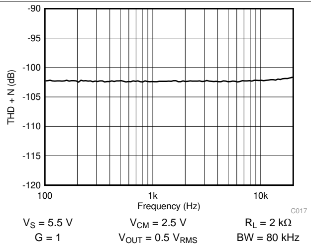
16. THD + N vs Frequency
