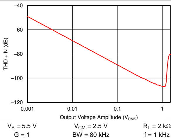
17. THD + N vs Amplitude
