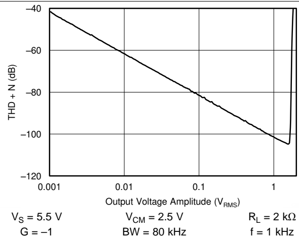
18. THD + N vs Amplitude
