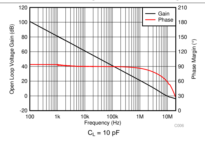
图 6. Open-Loop Gain and Phase vs Frequency
