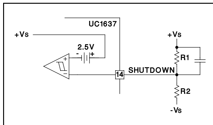
Figure 5. Delayed Start-Up
