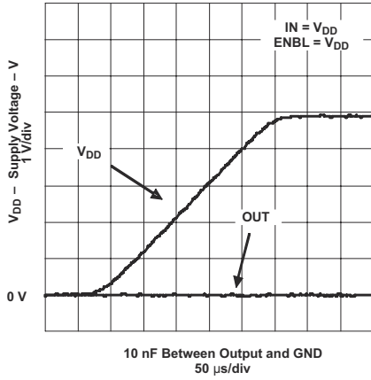
☒ 7-21. Output Behavior vs VDD (Inverting)
