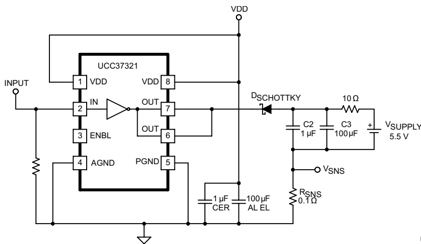
図 8-1. Sink Current Test Circuit
