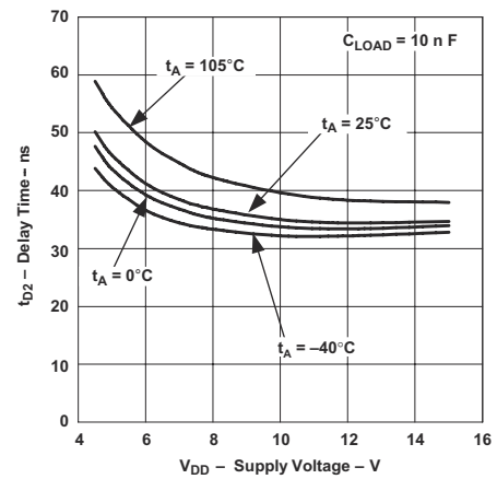
7-12. t_{D2} Delay Time vs Supply Voltage
