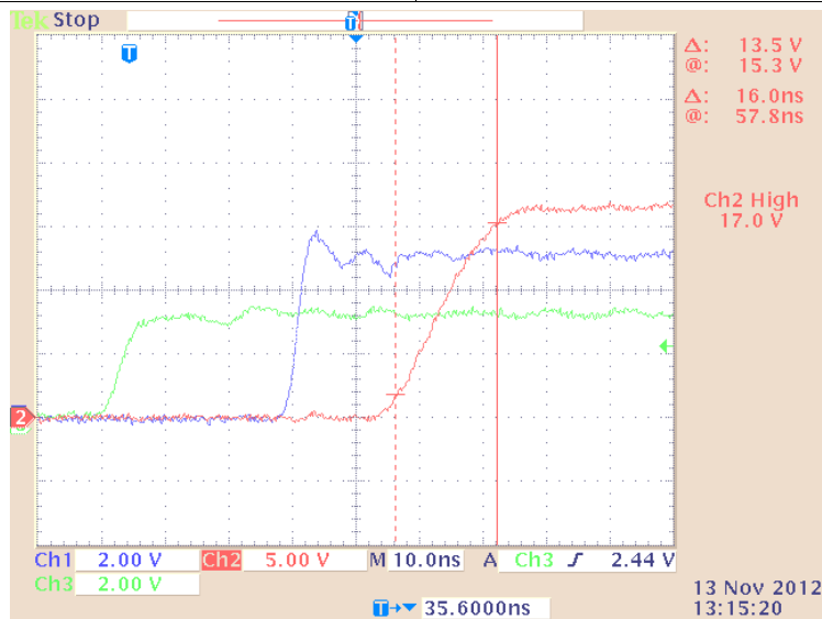
図 44. UCC27531DBV Input vs. Output PWM Rise Time
