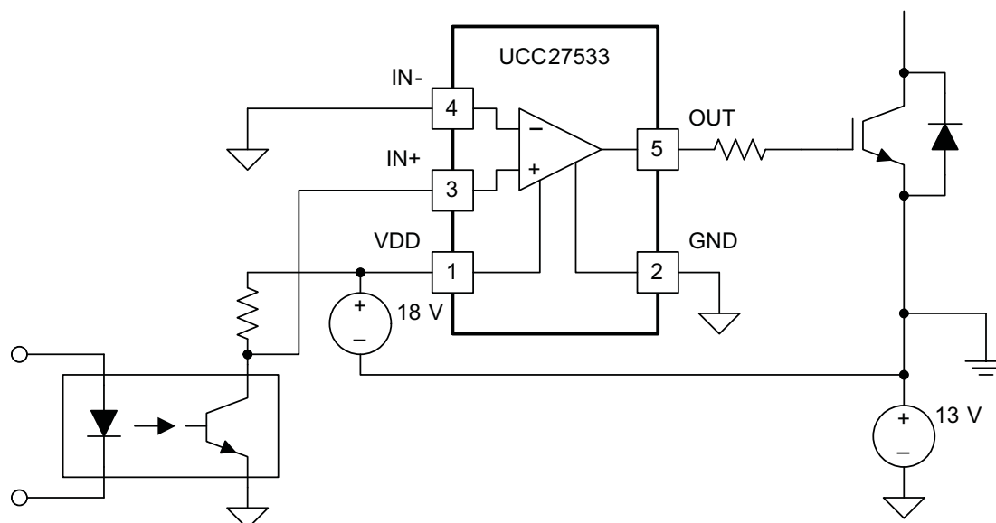
FIG 46. Single-Output Driver
