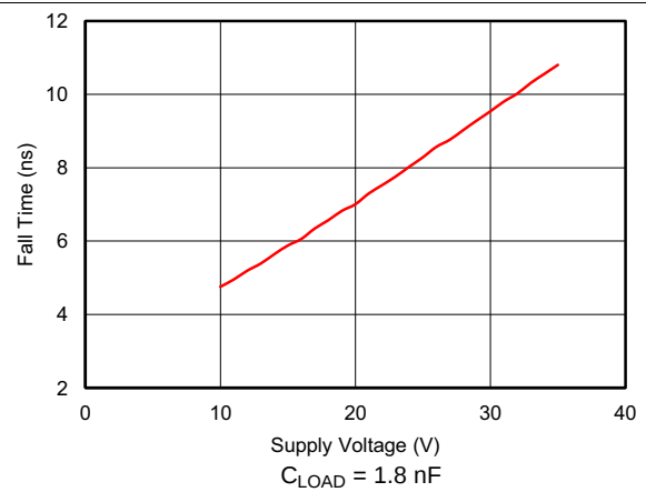
FIG 5. Fall Time vs. Supply Voltage
