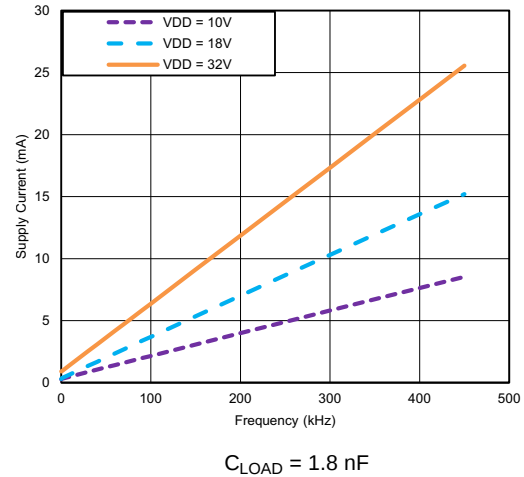
FIG 9. Operating Supply Current vs. Frequency
