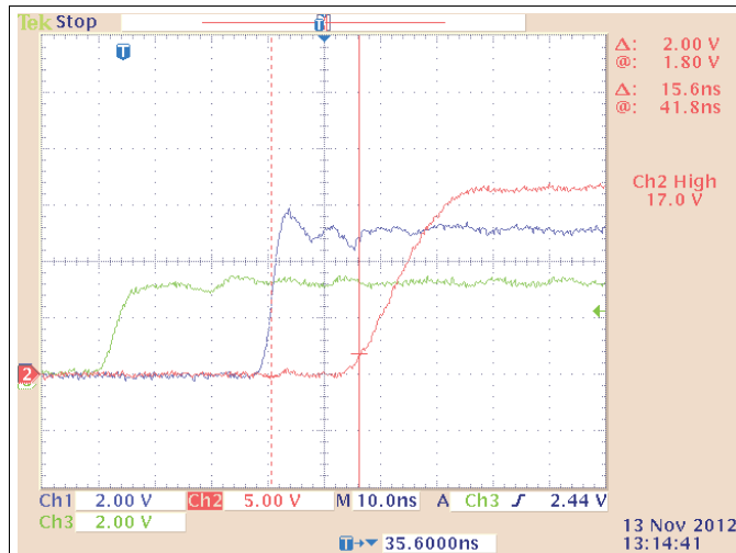
図 42. UCC27531DBV Input vs. Output PWM Propagation Delay (High)
