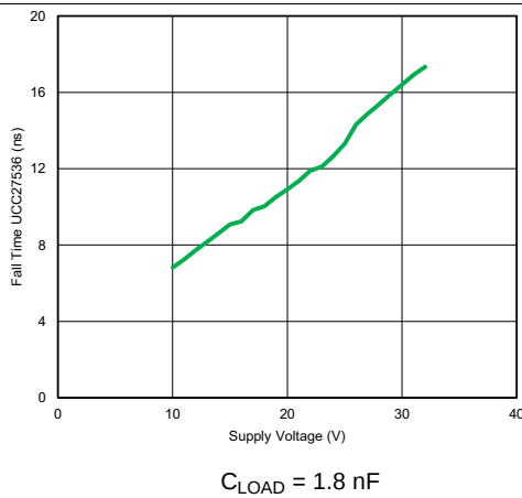
FIG 6. UCC27536 Fall Time vs. Supply Voltage
