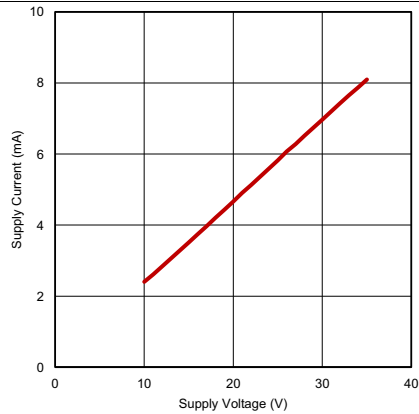
FIG 28. Operating Supply Current vs. Supply Voltage (Output Switching)
