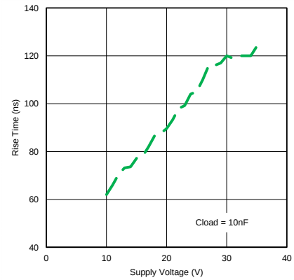
FIG 29. Rise Time vs. Supply Voltage
