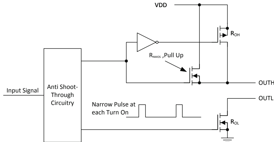
FIG 39. UCC27531 Gate Driver Output Stage
