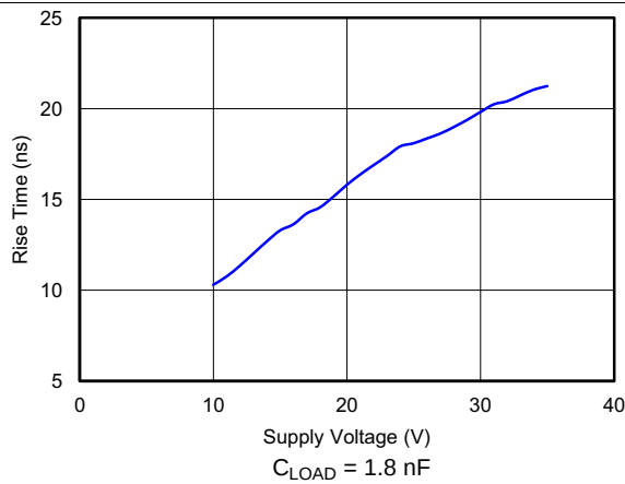
FIG 4. Rise Time vs. Supply Voltage
