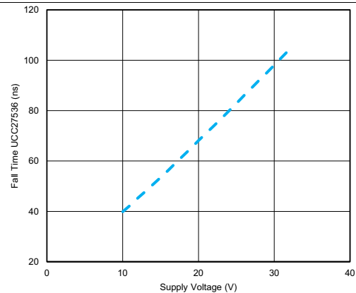
FIG 31. UCC27536 Fall Time vs. Supply Voltage
