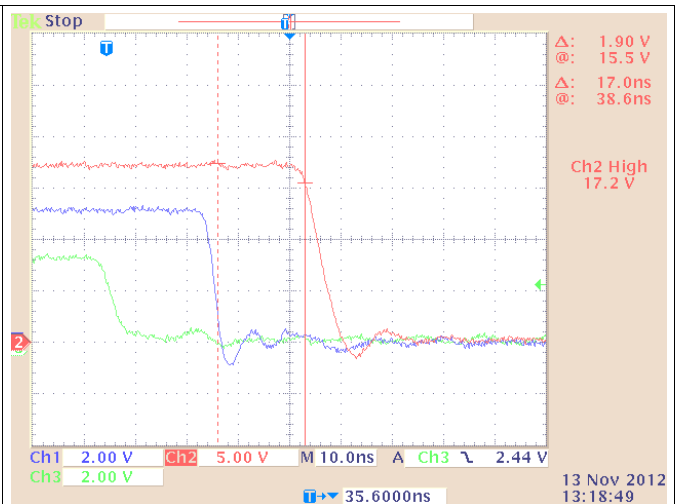
図 43. UCC27531DBV Input vs. Output PWM Propagation Delay (Low)
