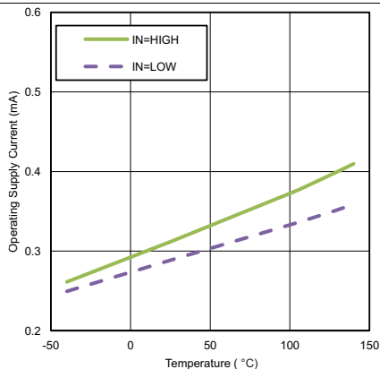
FIG 22. Operating Supply Current vs. Temperature (Output In DC On/Off Condition)
