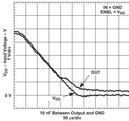
7-20. Output Behavior vs V_{DD} (UCC37321)
