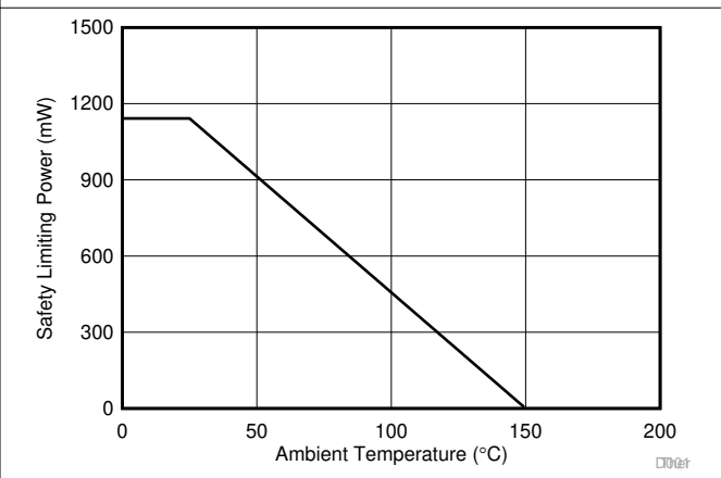
6-4. Thermal Derating Curve for Limiting Power per VDE for D Package
