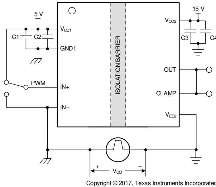
图 7-4. CMTI Test Circuit for Miller Clamp (UCC5350MC)
