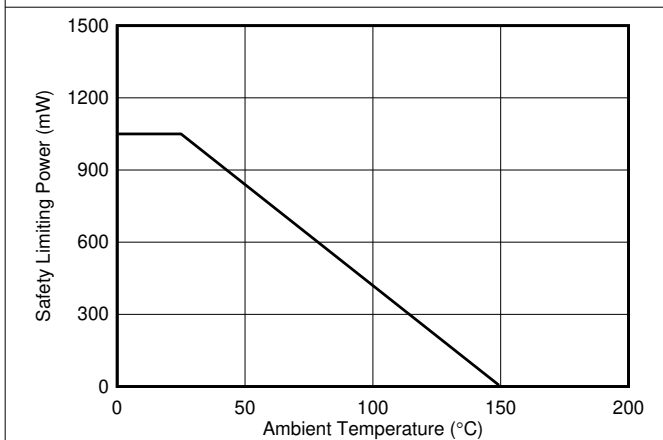
6-3. Thermal Derating Curve for Limiting Power per VDE for DWV Package
