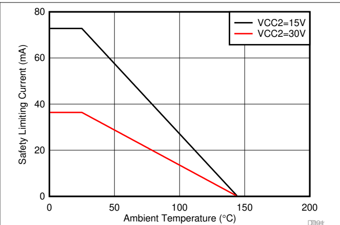
6-2. Thermal Derating Curve for Limiting Current per VDE for D Package
