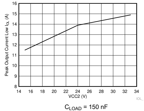
6-6. Output-Low Drive Current vs Output Voltage
