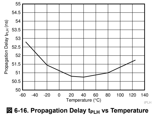
Figure 6-16. Propagation Delay tPLH vs Temperature
