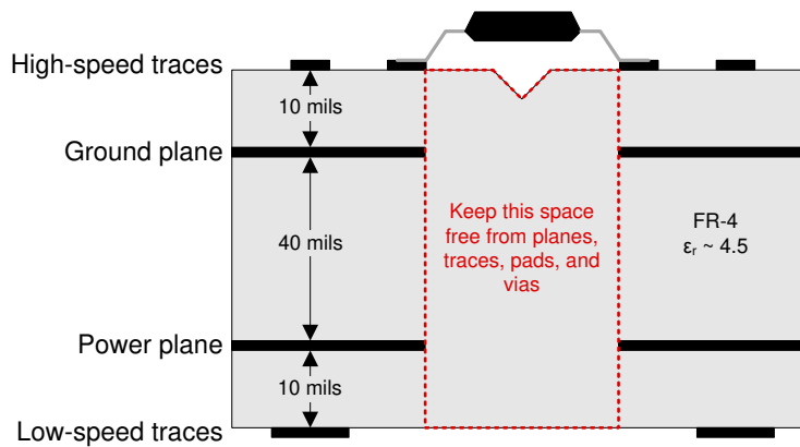
11-5. Recommended Layer Stack
