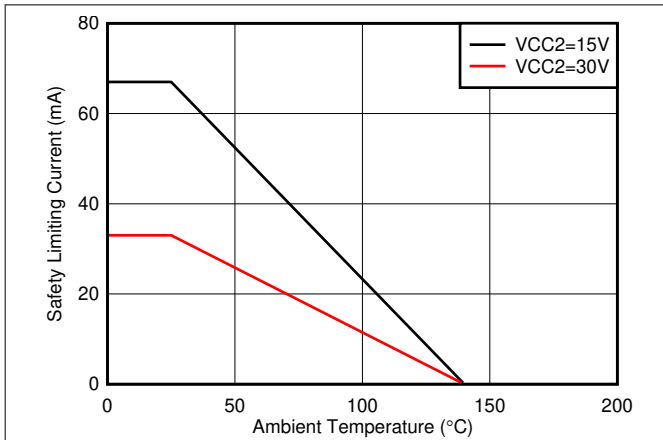
6-1. Thermal Derating Curve for Limiting Current per VDE for DWV Package
