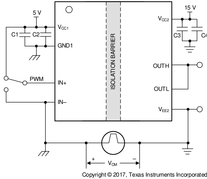
图 7-3. CMTI Test Circuit for Split Output (UCC5350SB)
