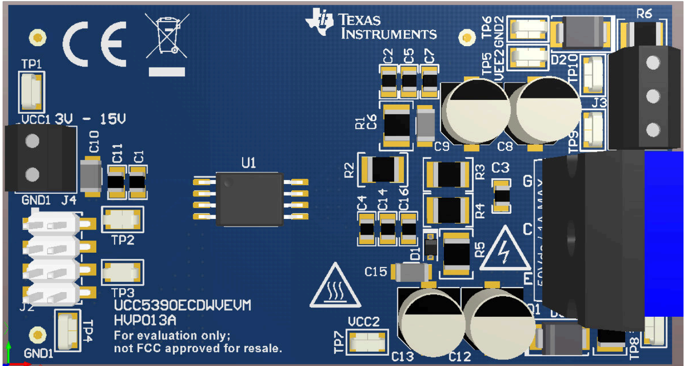
11-4. 3-D PCB View
