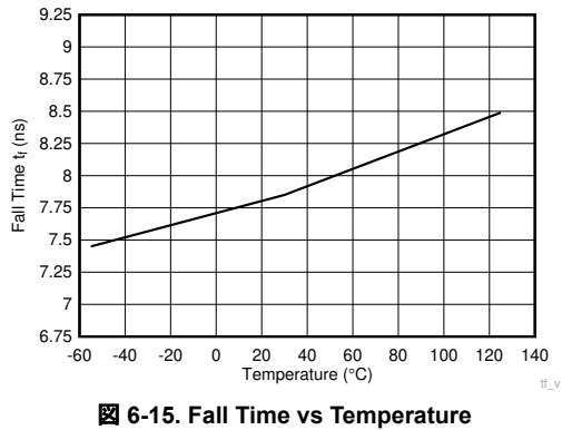
Figure 6-15. Fall Time vs Temperature
