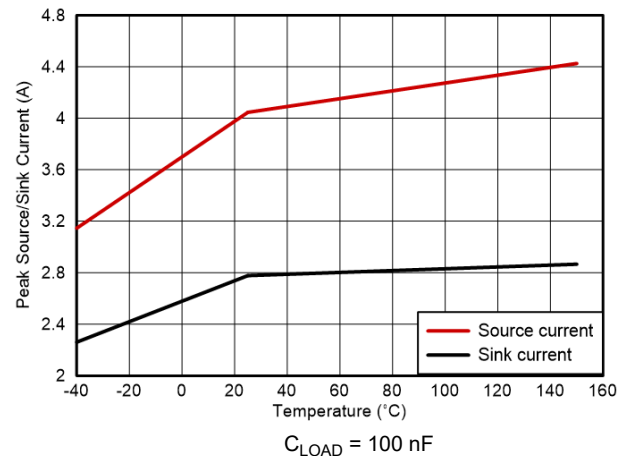
図 5-28. Peak Source and Sink Current
