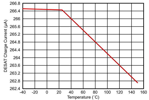
図 5-26. DESAT Charge Current vs Temperature
