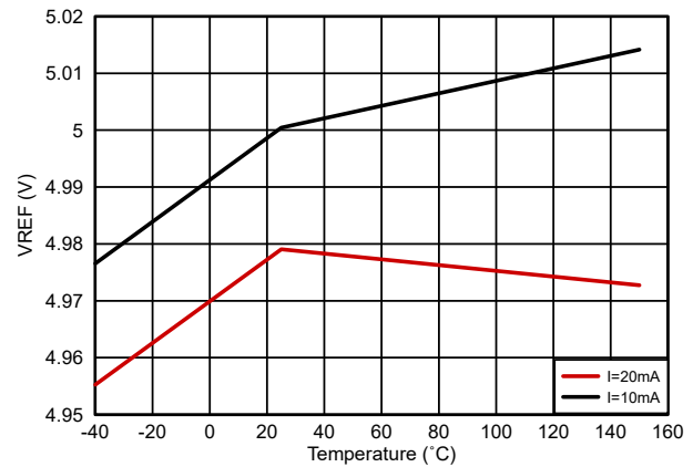
図 5-24. Vref Voltage vs Temperature
