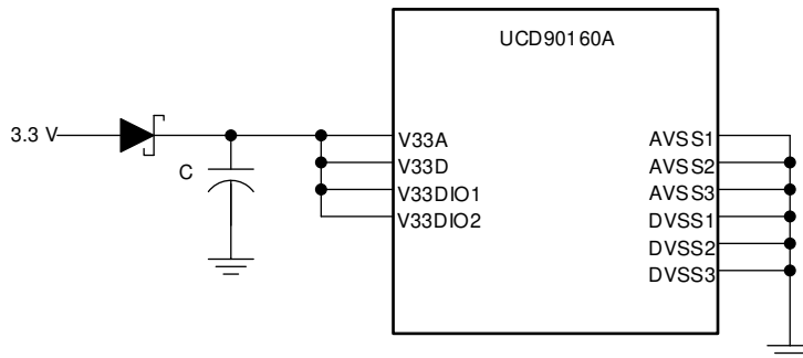
Figure 28. Brownout Circuit
