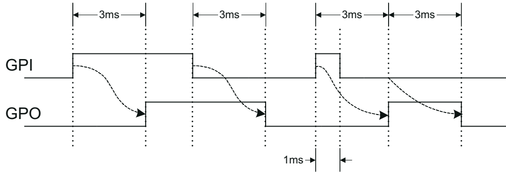
✎ 7-16. GPO Behavior When Ignoring Inputs During Delay
