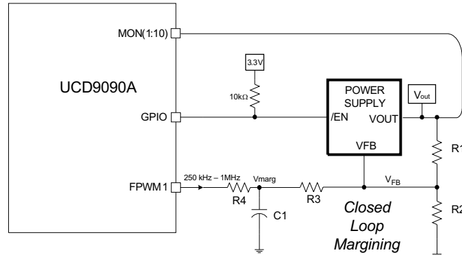
7-22. Closed-Loop Margining
