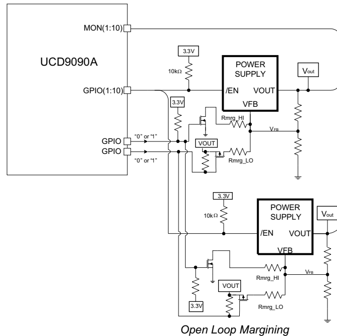
7-21. Open-Loop Margining
