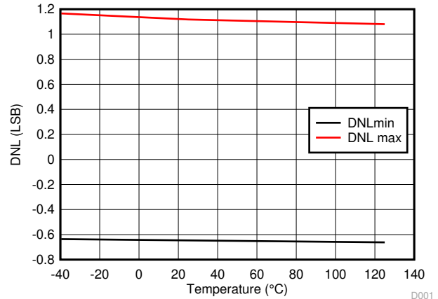
6-4. ADC Differential Nonlinearity vs Temperature
