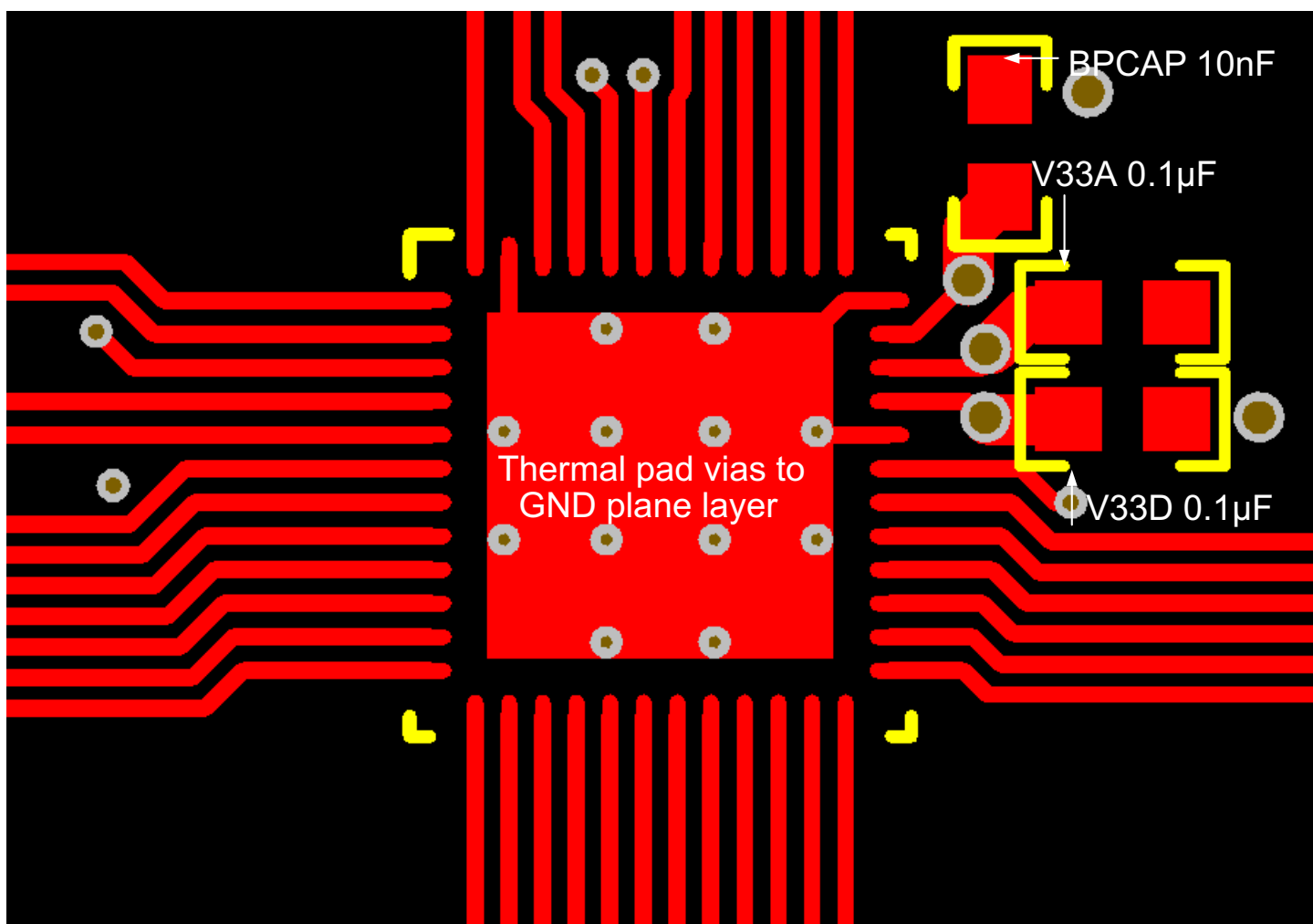
FIG 10-1. UCD9090A Layout Example, Top Layer
