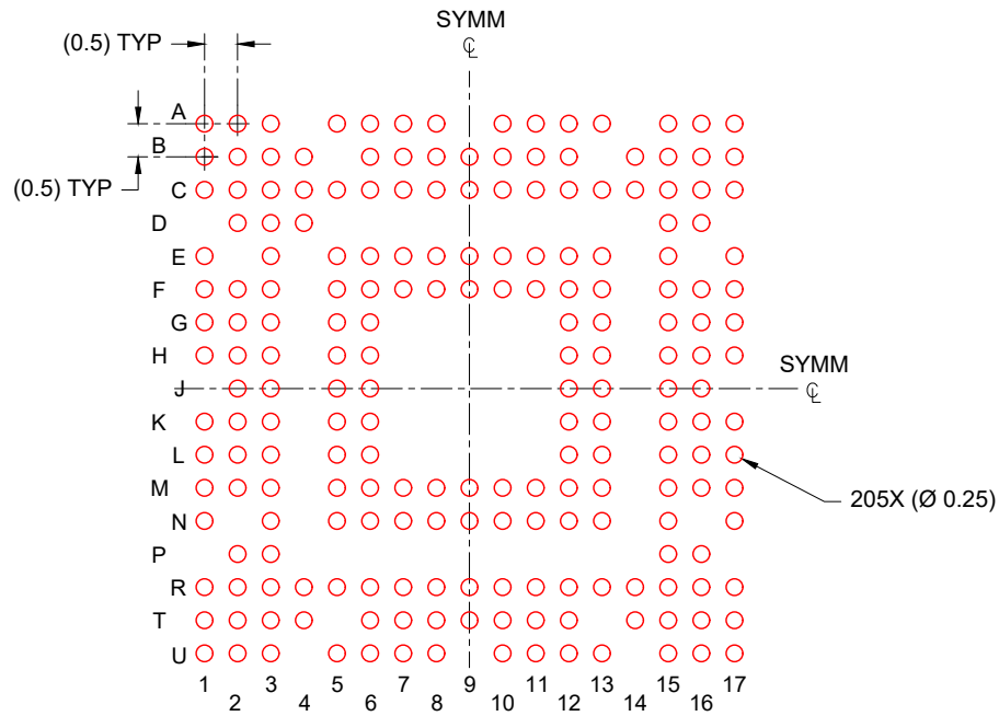
SOLDER PASTE EXAMPLE BASED ON 0.100 mm THICK STENCIL SCALE: 8X
