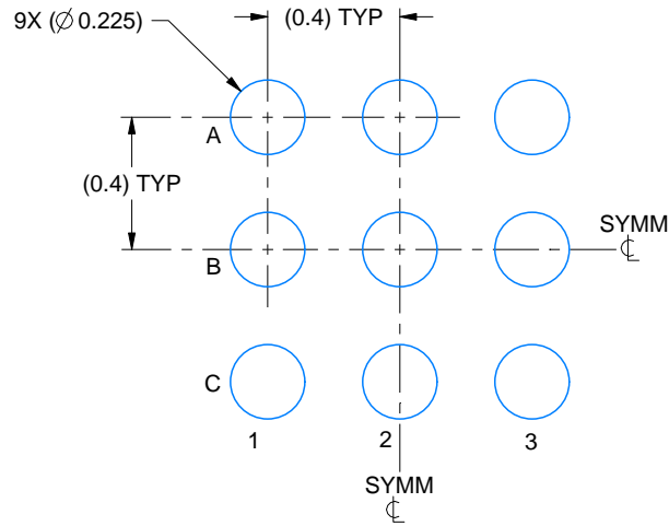
LAND PATTERN EXAMPLE SCALE:40X
