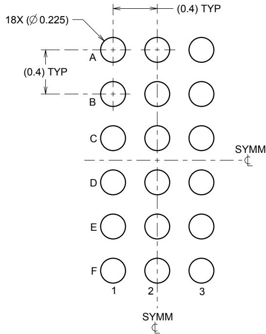
LAND PATTERN EXAMPLE SCALE:30X
