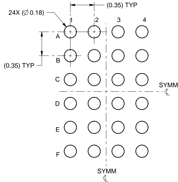
LAND PATTERN EXAMPLE SCALE:30X
