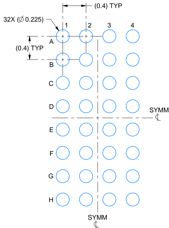
LAND PATTERN EXAMPLE EXPOSED METAL SHOWN SCALE:25X
