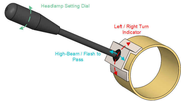
Figure 4. Multifunction Position Detection
