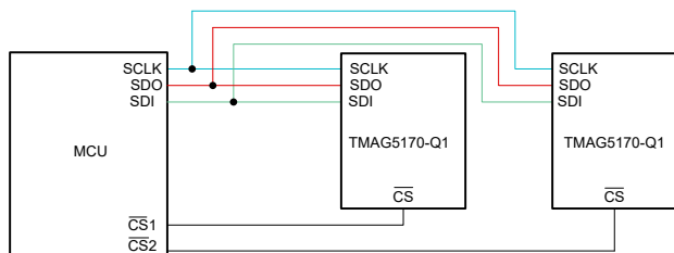
Figure 6. Simplified Block Diagram
