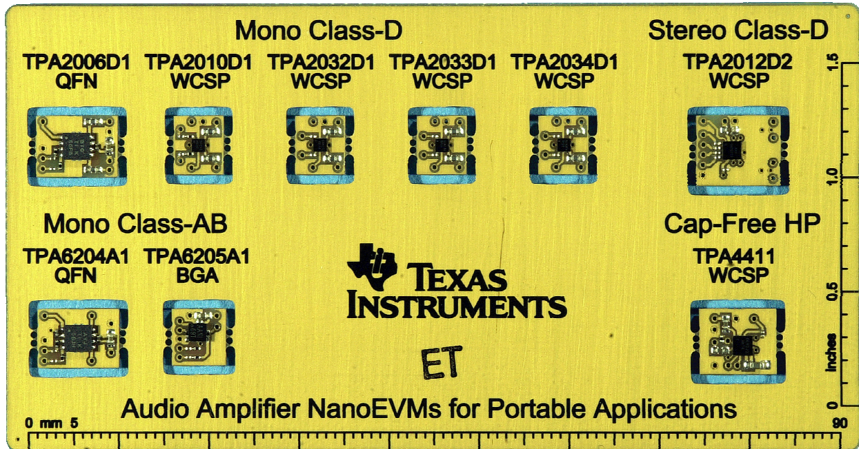
Nano-Evaluation Module – Top Side View
