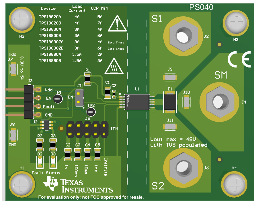
TPSI88XXEVM
