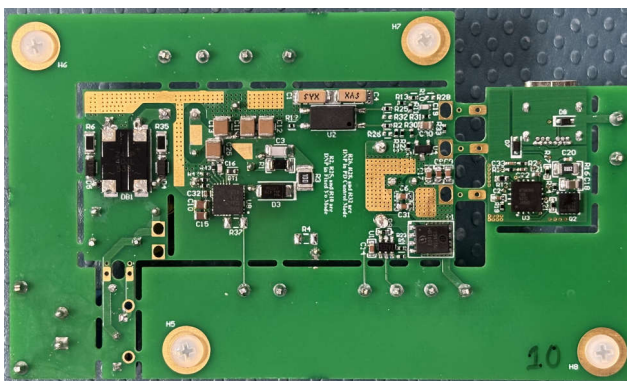
UCG28836EVM-150 (底面図)
