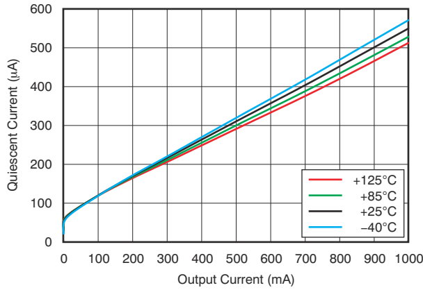
6-7. Quiescent Current vs Load
