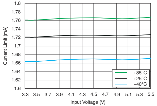
6-8. Current Limit vs Input Voltage
