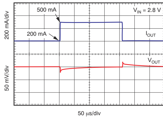
6-14. Load Transient Response 200 mA to 500 mA
