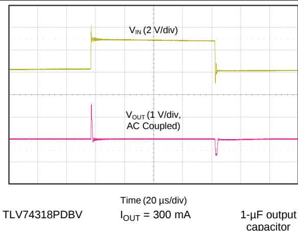
FIG 24. Line Transient
