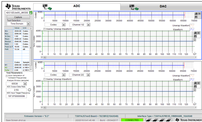
図 189. Idle-Channel Noise (No Input) for 2.5-GSPS, Dual-Channel Oscilloscope
