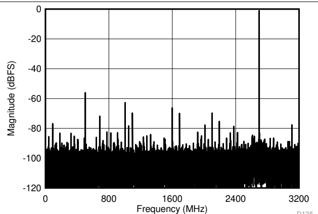
Figure 21. Single-Tone FFT at A_{\text{IN}} = -1\text{ dBFS}
