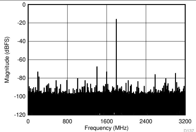
Figure 29. Single-Tone FFT at A_{\text{IN}} = -16\text{ dBFS}
