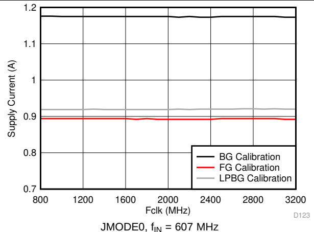
Figure 53. IA19 Supply Current vs Clock Frequency
