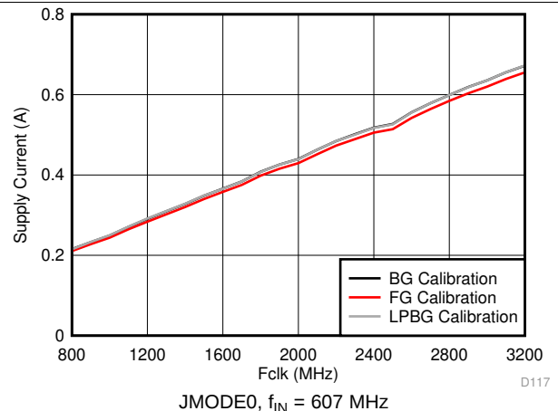
Figure 55. ID11 Supply Current vs Clock Frequency
