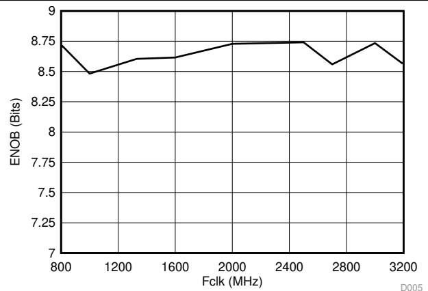
Figure 15. ENOB vs Clock Frequency
