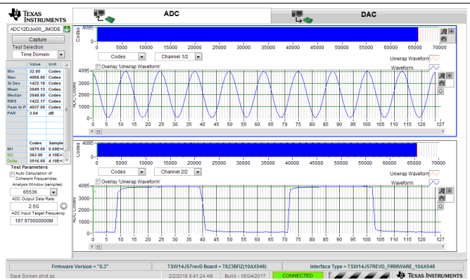
図 190. 200-MHz, Sine-Wave (Channel A) and 40-MHz, Square-Wave (Channel B) Time Domain for 5-GSPS, Single-Channel Oscilloscope
