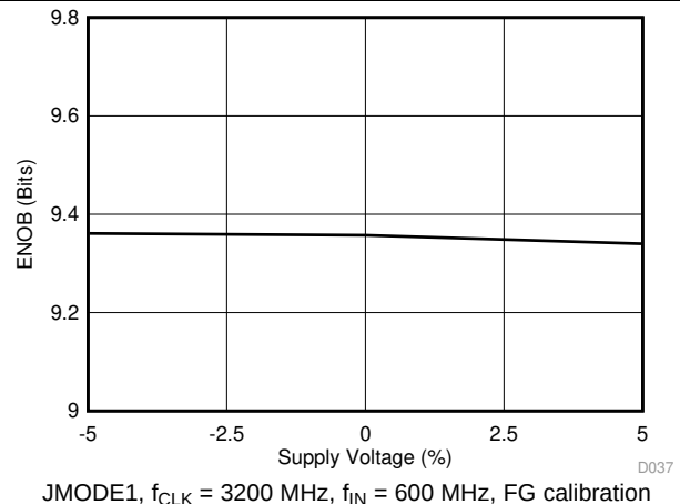
Figure 41. ENOB vs Supply Voltage
