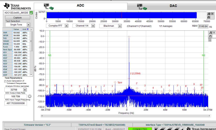
182. FFT for 497.77-MHz Input Signal, 2.7 GSPS, JMODE2
