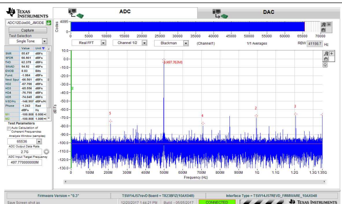
182. FFT for 497.77-MHz Input Signal, 2.7 GSPS, JMODE2
