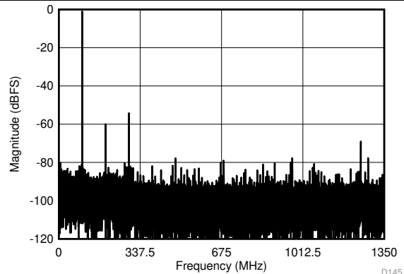
Figure 24. Single-Tone FFT at A_{\text{IN}} = -1\text{ dBFS}
