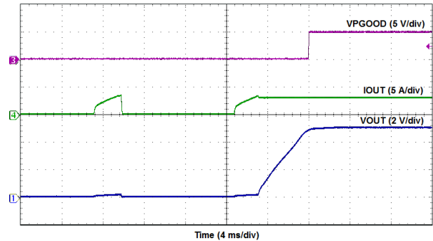
7-16. Removal of Overcurrent
