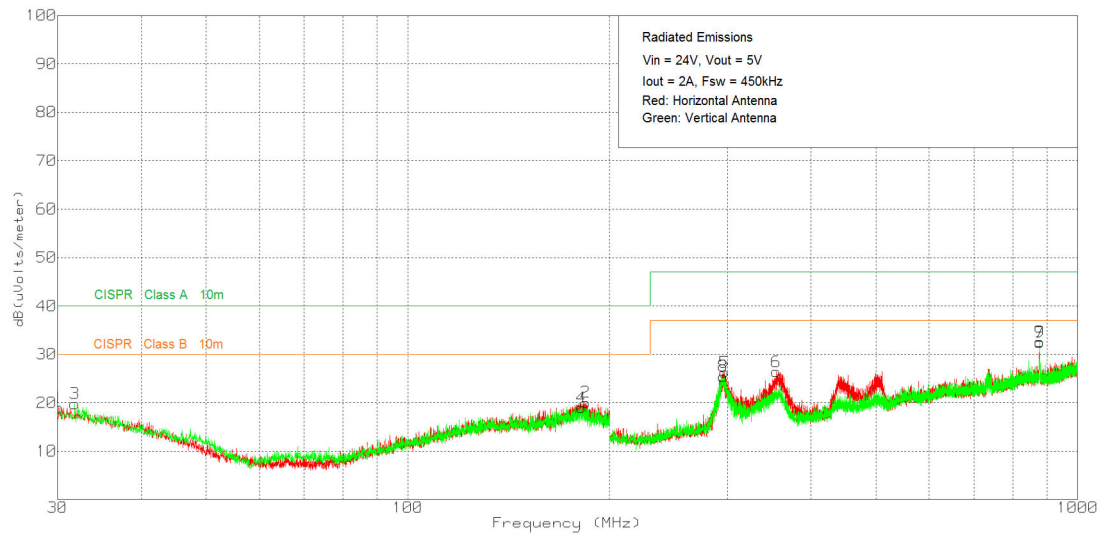
图 9-6. Radiated Emissions 24-V Input, 5-V Output, 2-A Load (EN55011 Class B)
