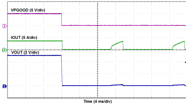
7-15. Overcurrent Limiting
