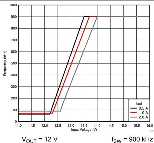
7-7. Frequency Foldback
