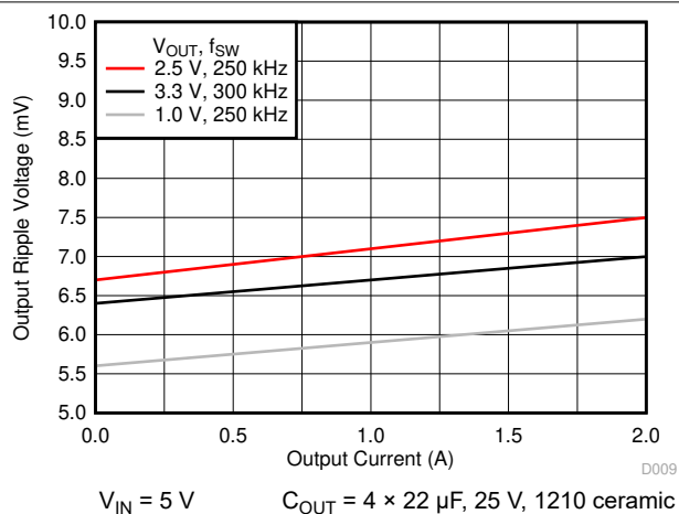
6-3. Voltage Ripple vs Output Current
