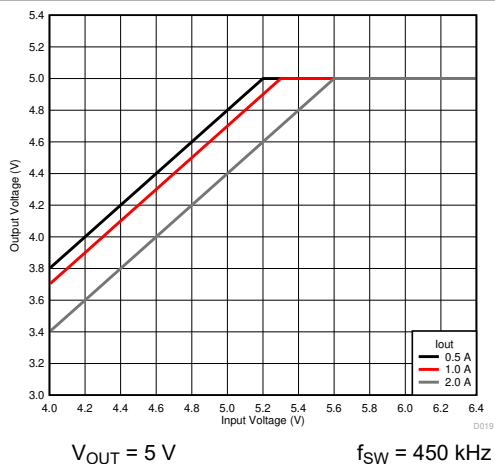
7-4. Voltage Dropout
