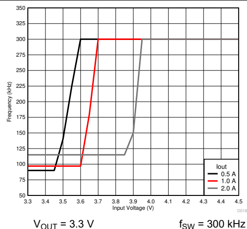
7-3. Frequency Foldback
