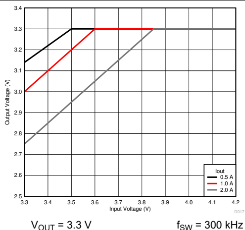
7-2. Voltage Dropout
