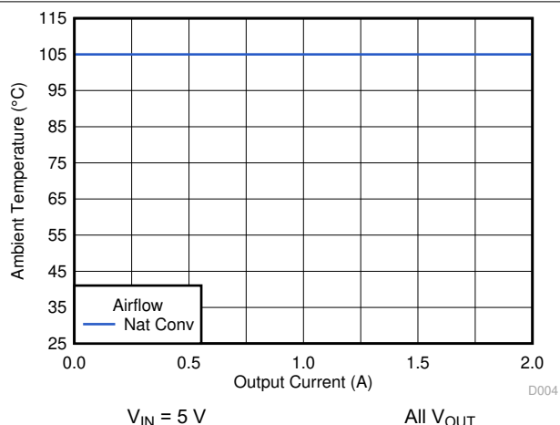
6-4. Safe Operating Area
