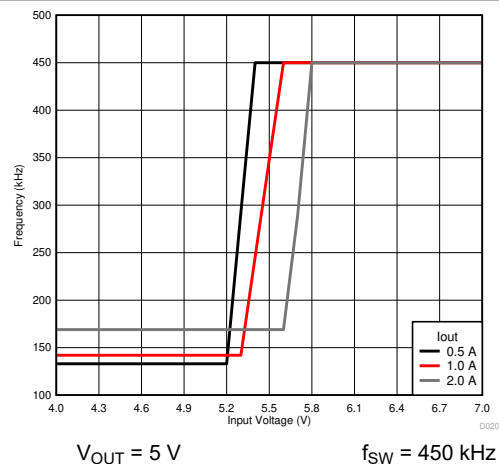
7-5. Frequency Foldback
