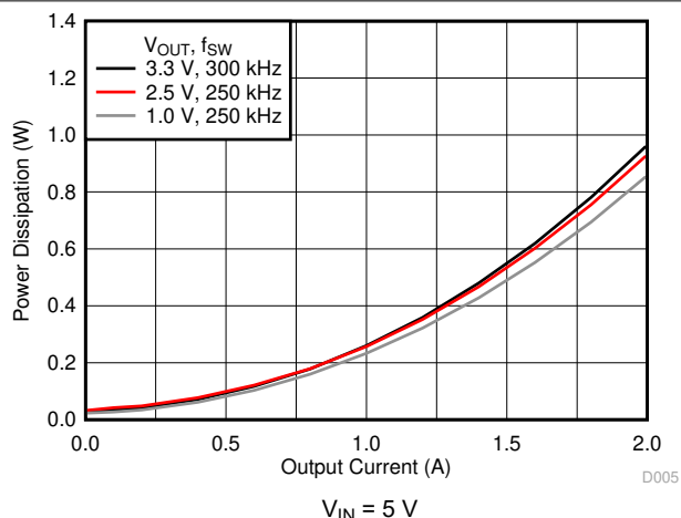
6-2. Power Dissipation vs Output Current
