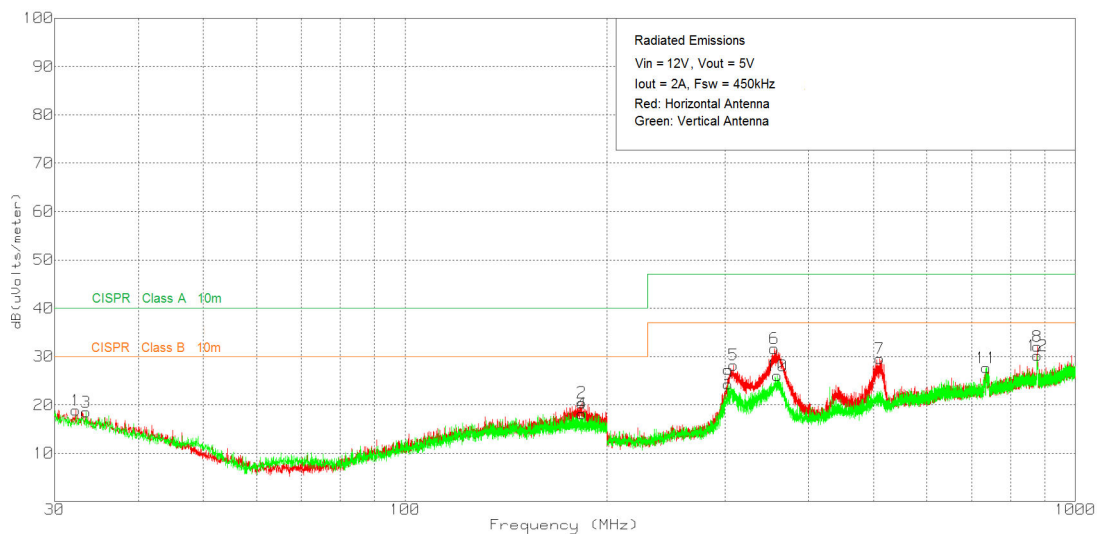
图 9-8. Radiated Emissions 12-V Input, 5-V Output, 2-A Load (EN55011 Class B)
