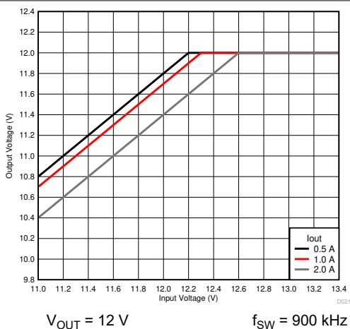
7-6. Voltage Dropout
