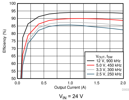
6-9. Efficiency vs Output Current
