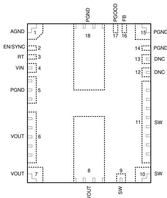
FIG 5-1. RLR Package 18-Pin QFN Top View
