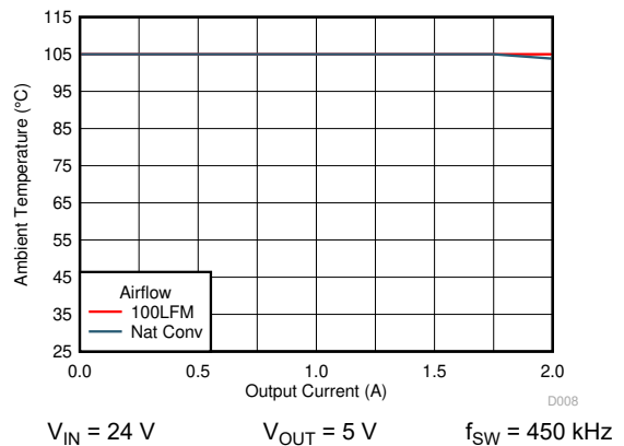
6-12. Safe Operating Area
