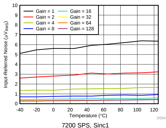
Figure 19. Noise vs Temperature
