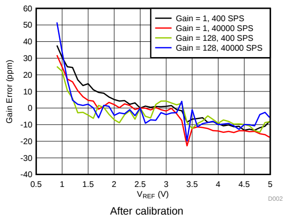
Figure 17. Gain Error vs Reference Voltage
