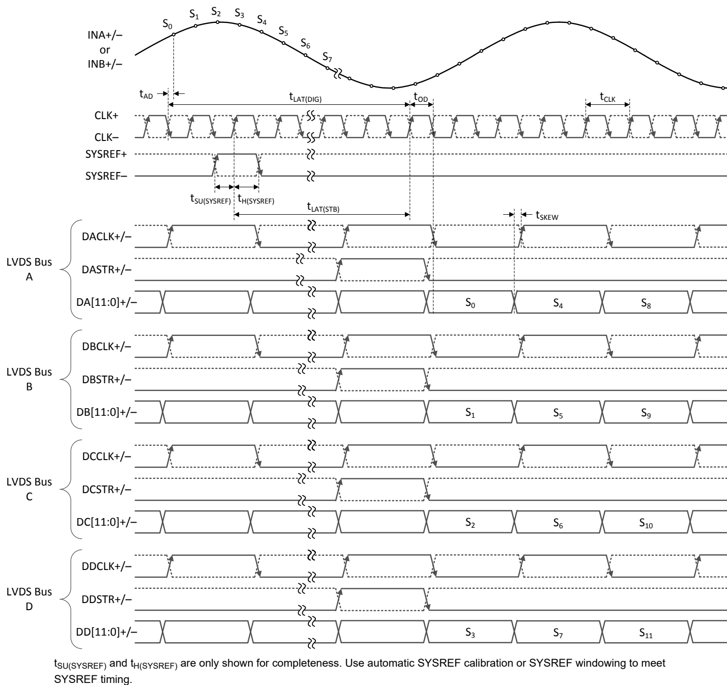
6-7. Single-Channel, 4-Bus, Aligned-Mode Timing (LDEMUX = 1, DES_EN = 1, LALIGNED = 1)
