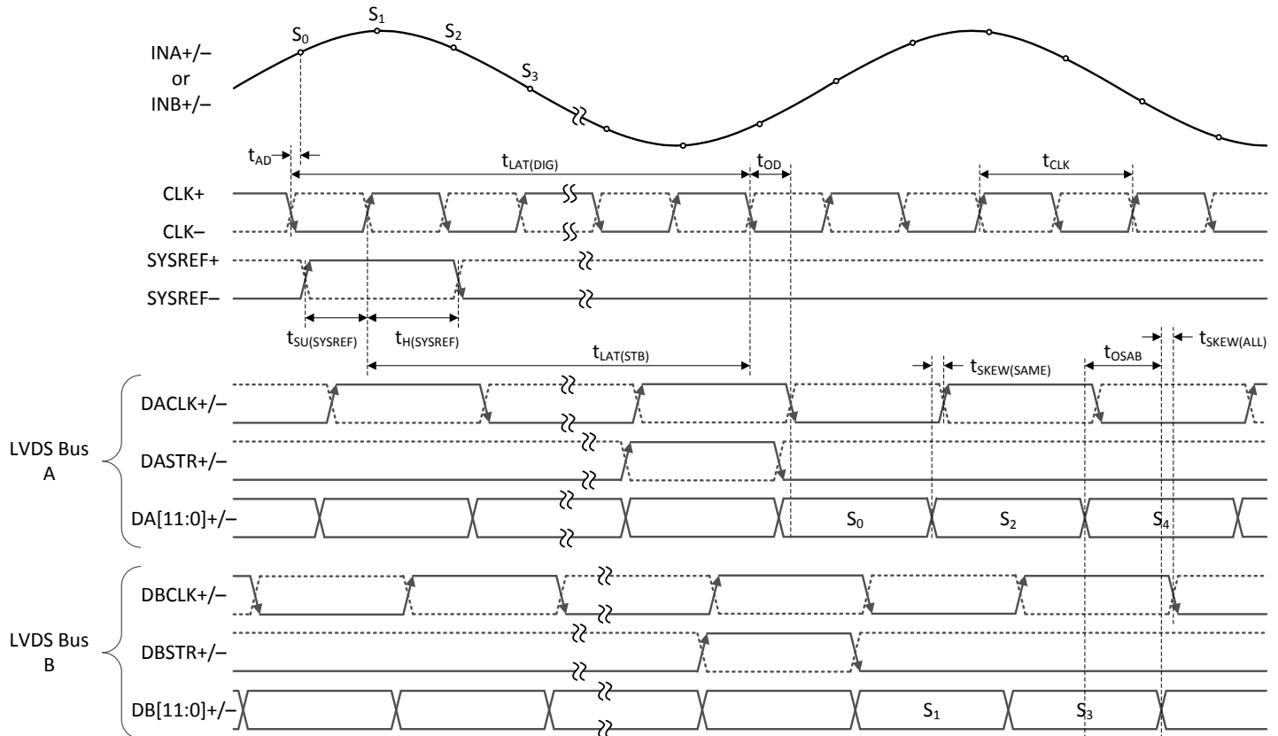
FIG 6-4. Single-Channel, 2-Bus, Staggered-Mode Timing (LDEMUX = 0, DES_EN = 1, LALIGNED = 0)
