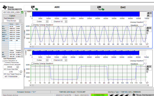
8-10. 200-MHz, Sine-Wave (Channel A) and 40-MHz, Square-Wave (Channel B) Time Domain for 5-GSPS, Single-Channel Oscilloscope
