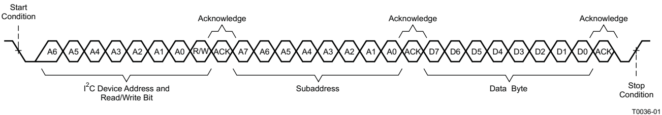
Figure 12. Write Transfer
