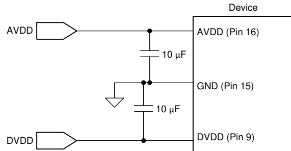
8-5. Power-Supply Decoupling
