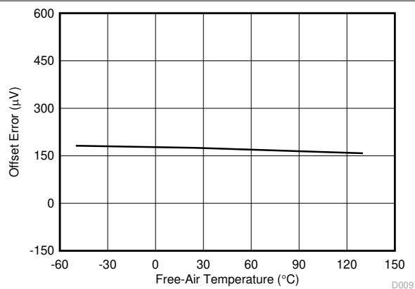
FIG 6-12. Offset Error vs Temperature
