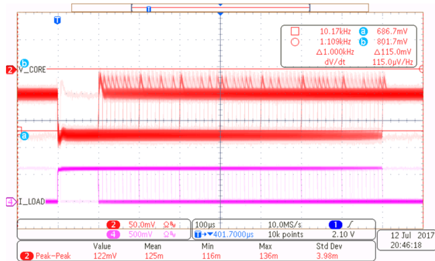
図 14. Core Rail — 90-A to 240-A Transient, 10% to 80% Duty Cycle Sweep
