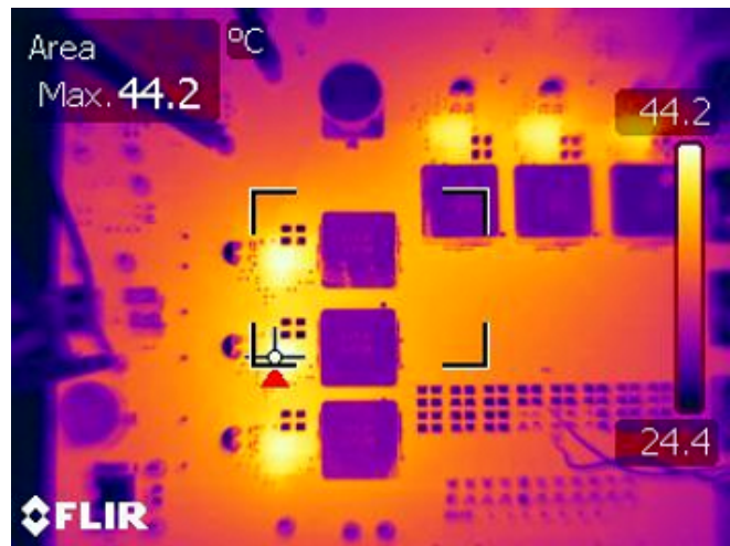
図 23. CSD95490Q5MC Temperature 100-A Load, 500-ft/min Airflow
