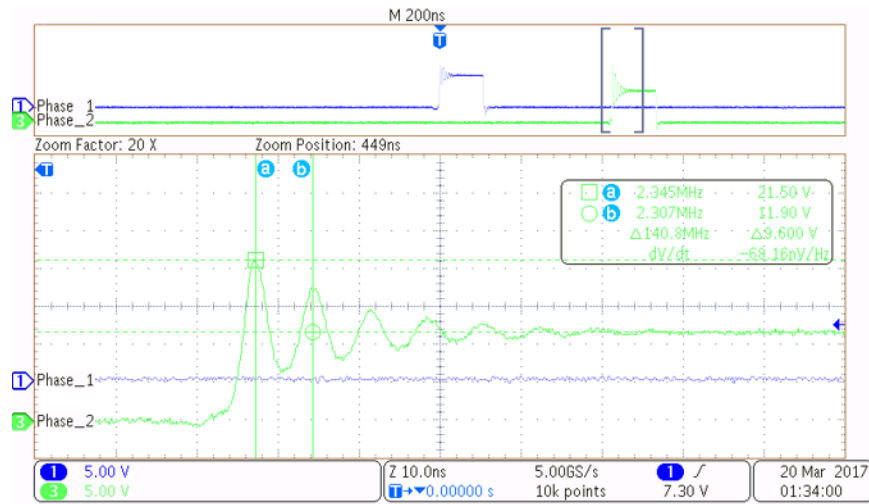
図 10. Phase Ringing — 200 A, No Snubber or Boot Resistor
