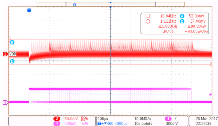
図 17. Auxiliary Rail — 10-A to 20-A Transient, 10% to 80% Duty Cycle Sweep
