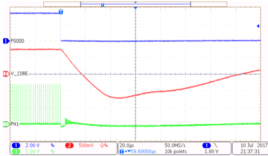
図 27. Overcurrent Shutdown
