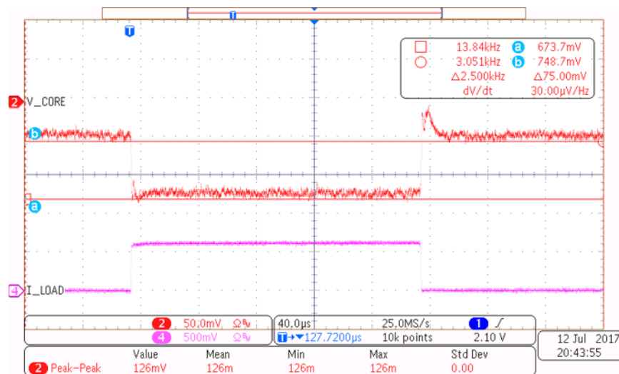
Fig 12. Core Rail — 90-A to 240-A Transient Undershoot, 20% Duty Cycle
