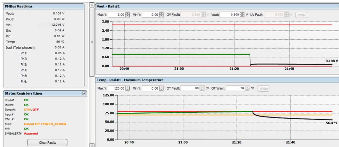
図 30. Overtemperature Shutdown as Seen in Fusion GUI
