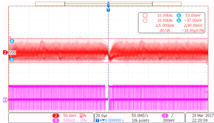
図 18. Auxiliary Rail — 10-A to 20-A Transient, 10-kHz to 200-kHz Load Frequency Sweep
