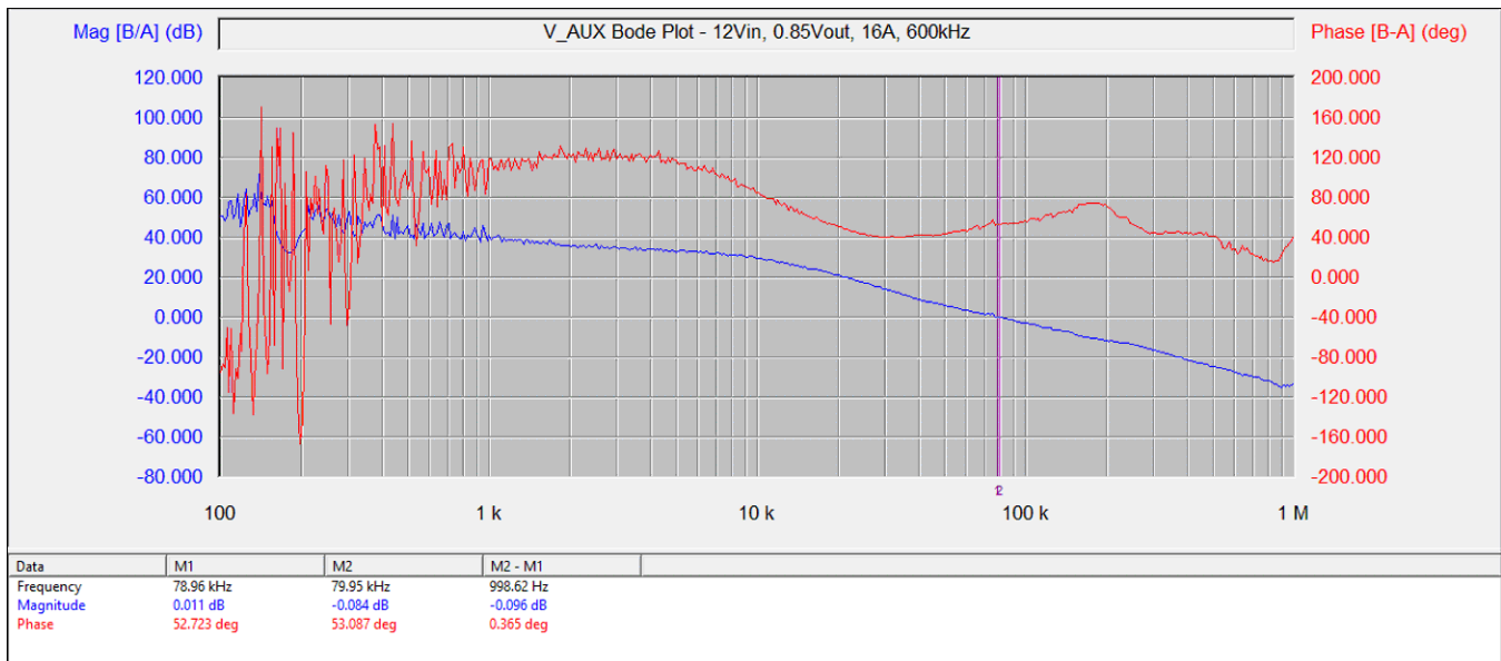
Figure 21. Auxiliary Rail Bode Plot
