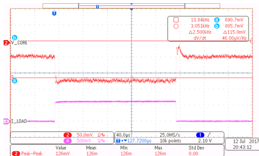
Fig 13. Core Rail — 90-A to 240-A Transient Overshoot, 20% Duty Cycle
