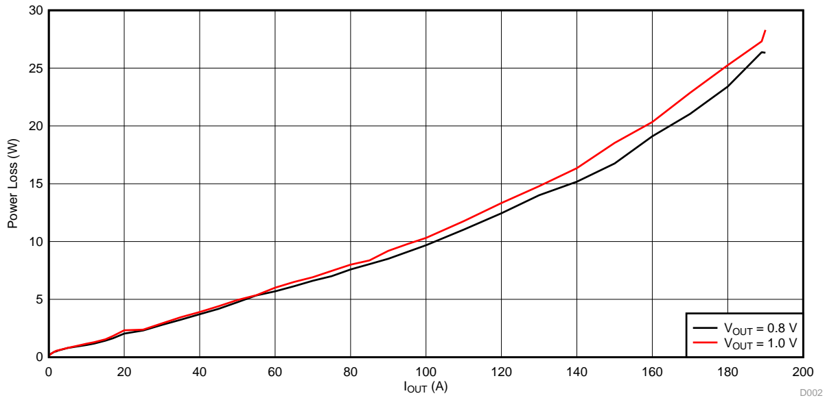
図 3. Core Rail Power Loss
