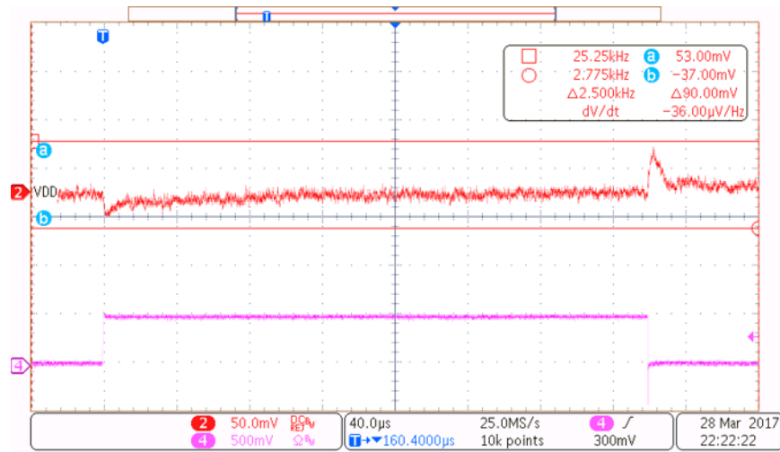
図 16. Auxiliary Rail — 10-A to 20-A Transient, 30% Duty Cycle
