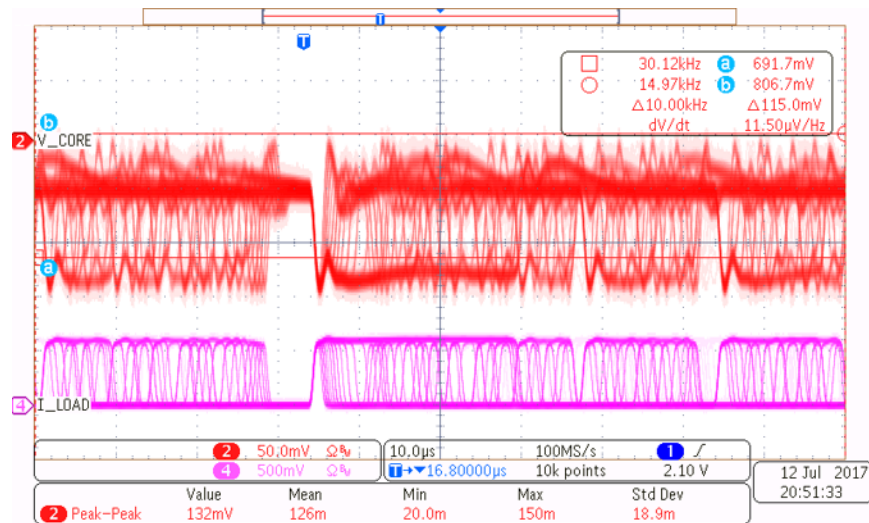
図 15. Core Rail — 90-A to 240-A Transient, 10-kHz to 200-kHz Load Frequency Sweep
