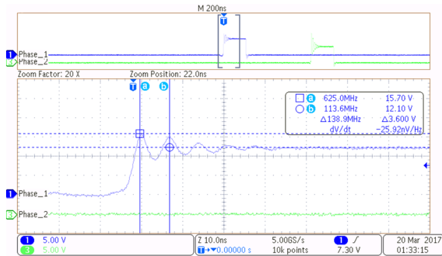
図 11. Phase Ringing — 200-A, 2-Ω Boot Resistor
