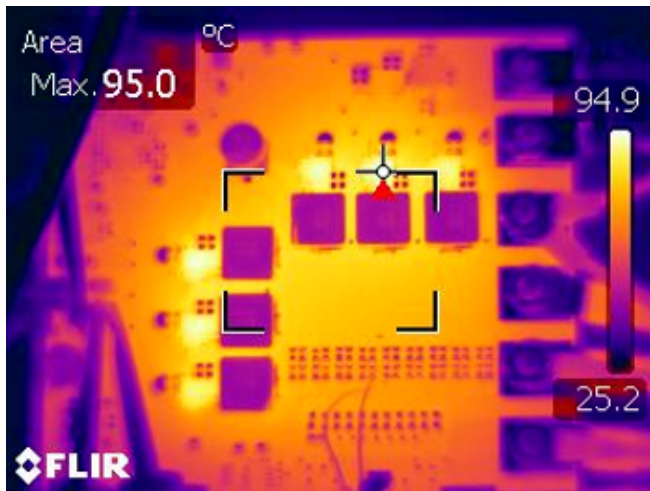
図 24. CSD95490Q5MC Temperature 200-A Load, No Airflow
