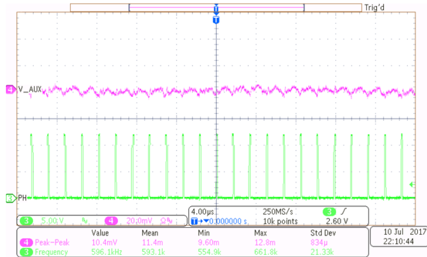
図 8. Auxiliary Rail — Steady State, 16 A
