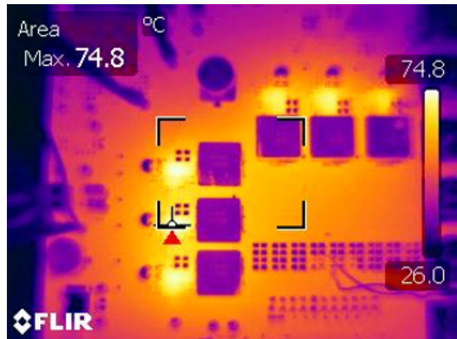
図 25. CSD95490Q5MC Temperature 200-A Load, 500-ft/min Airflow
