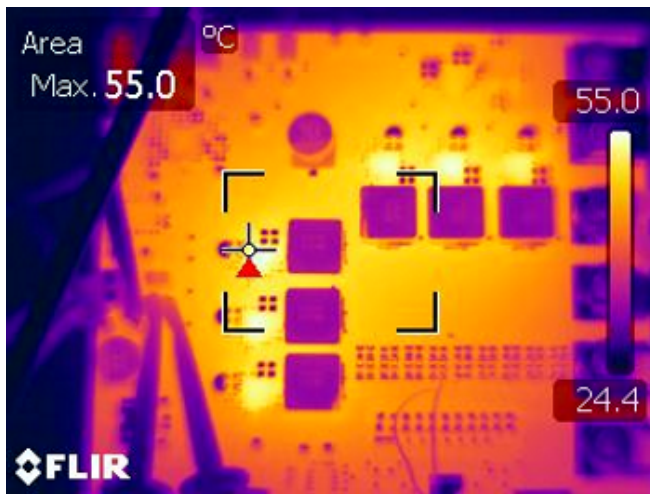
図 22. CSD95490Q5MC Temperature 100-A Load, No Airflow
