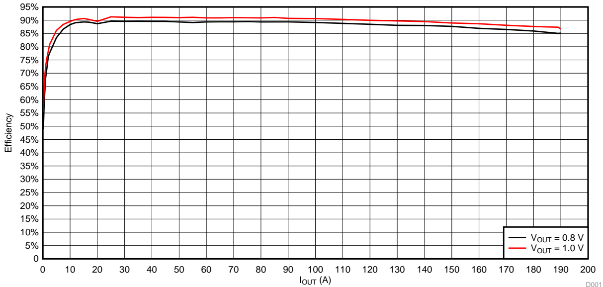
図 2. Core Rail Efficiency
