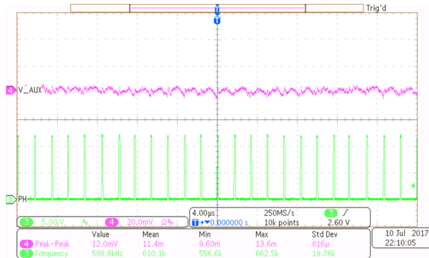
図 9. Auxiliary Rail — Steady State, 20 A
