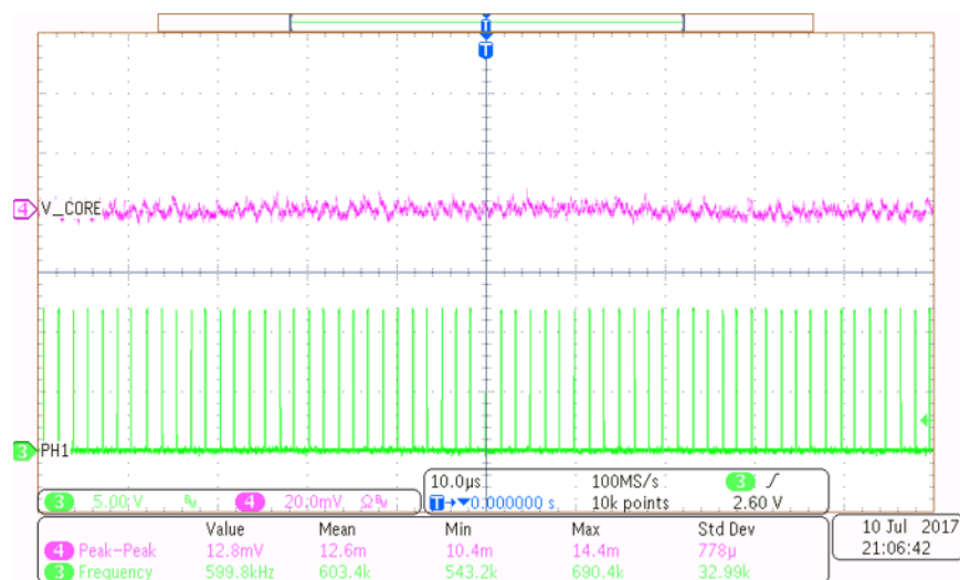
Figure 7. Core Rail — Steady State, 200 A
