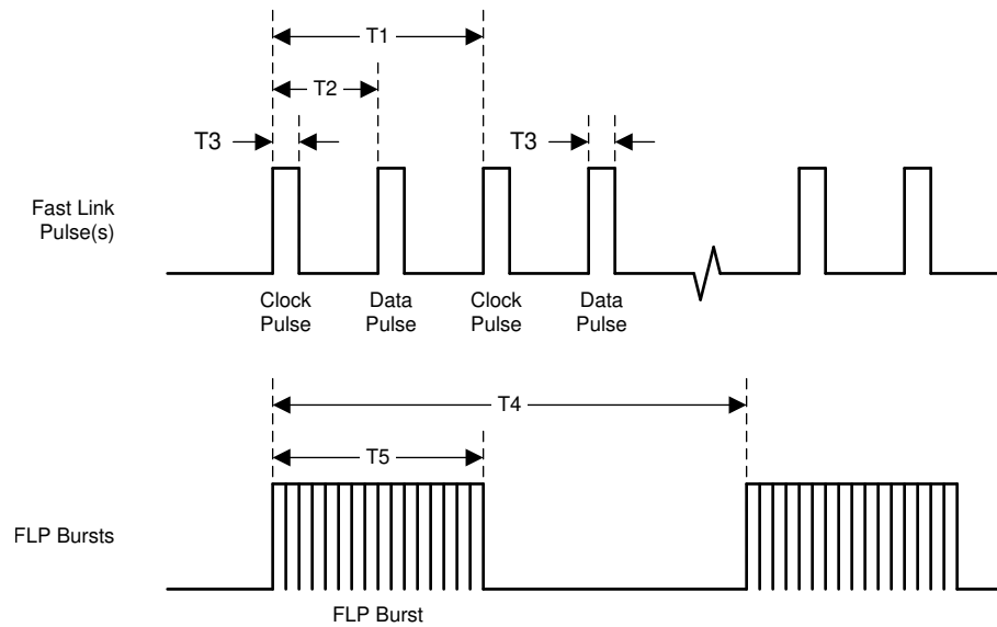
7-14. Fast Link Pulse Timing
