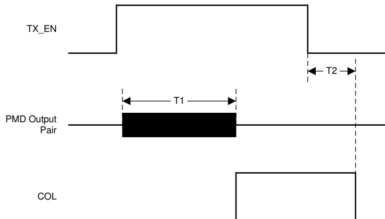
7-15. 10BASE-T Jabber Timing
