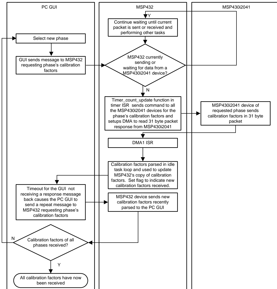
図 15. Process for Obtaining All Calibration Factors
