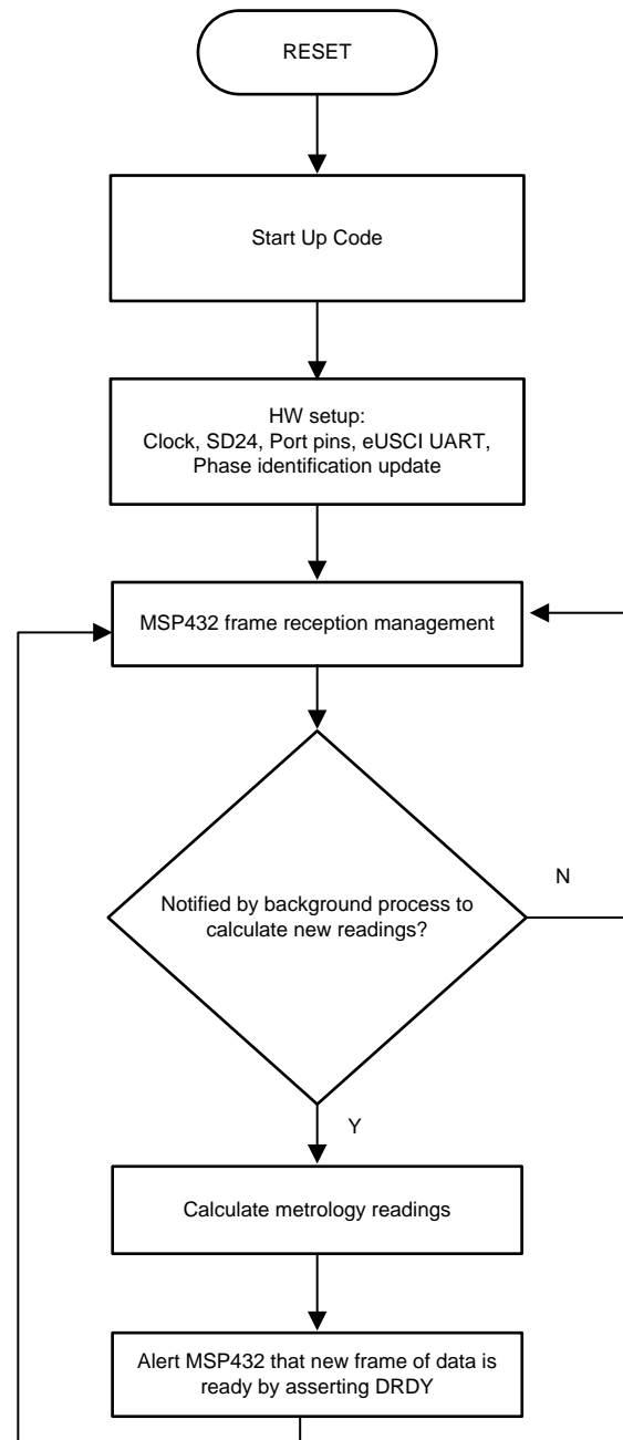
図 9. Metrology Foreground Process
