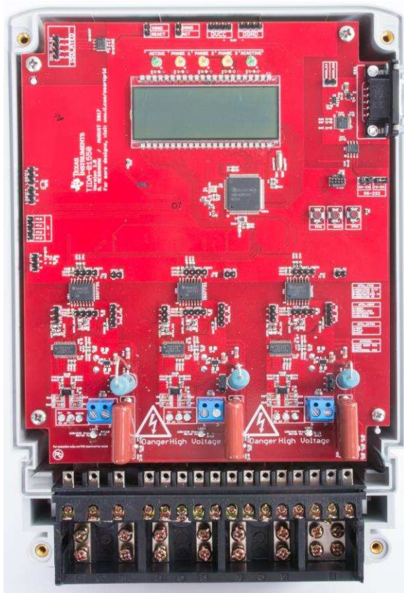
Figure 17. Top View of Reference Design
