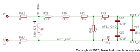
Figure 6. MSP430i2041 Voltage Front-End Circuitry
