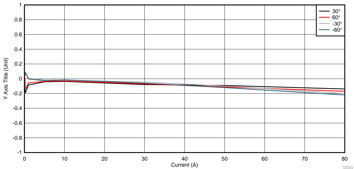
図 39. Cumulative Reactive Energy % Error Versus Current
