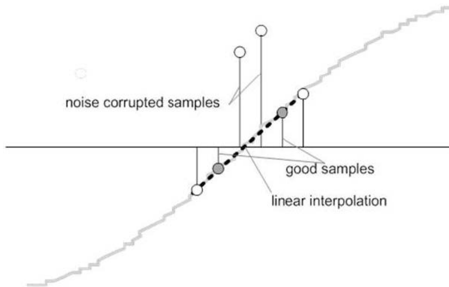
図 11. Frequency Measurement
