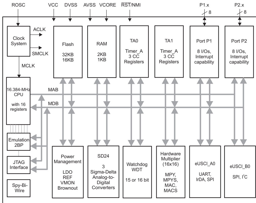
図 3. Functional Block Diagram of MSP430i2041
