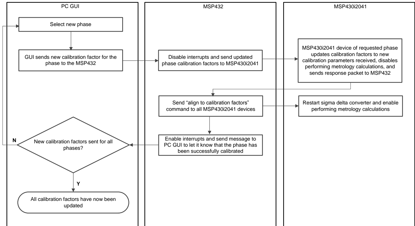
16. Process for Setting New Calibration Factors
