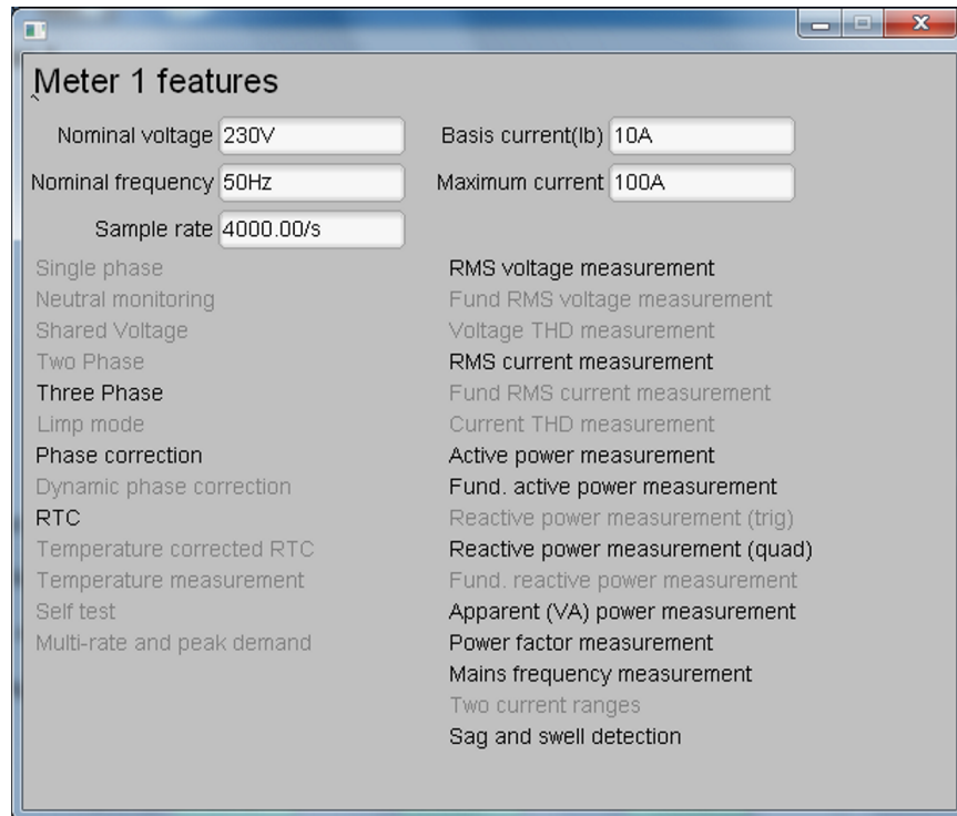
Figure 36. Meter Features Window
