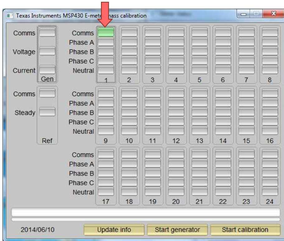
Figure 31. GUI Startup Window
