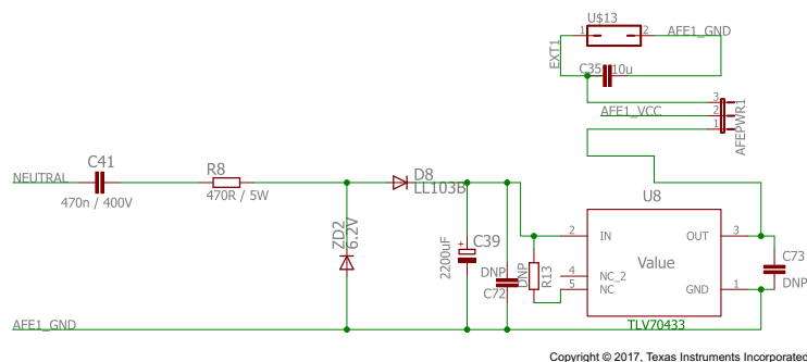
Figure 4. High-Side Power Supply
