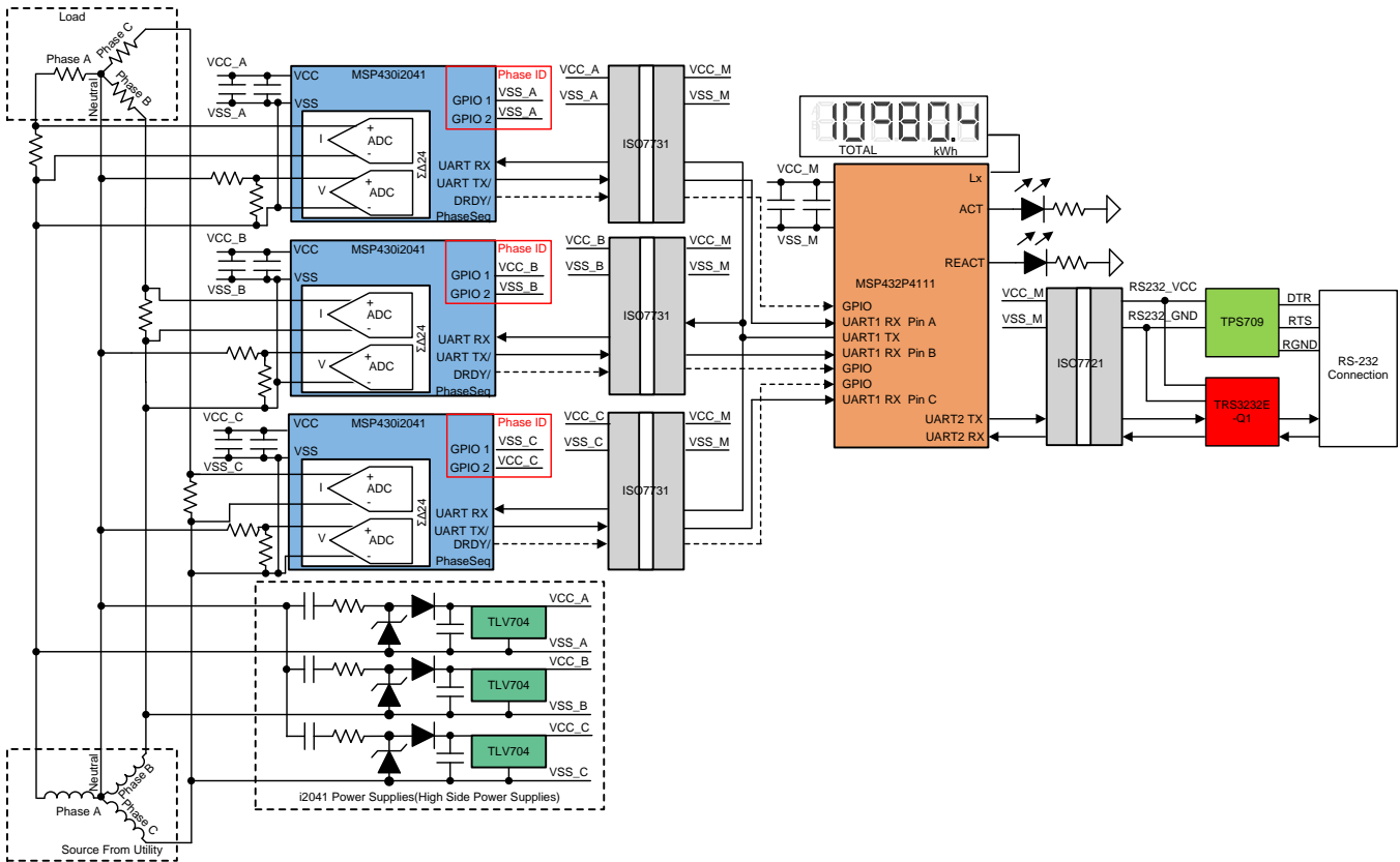
図 1. TIDA-01550 Block Diagram, Three Isolated Channels
