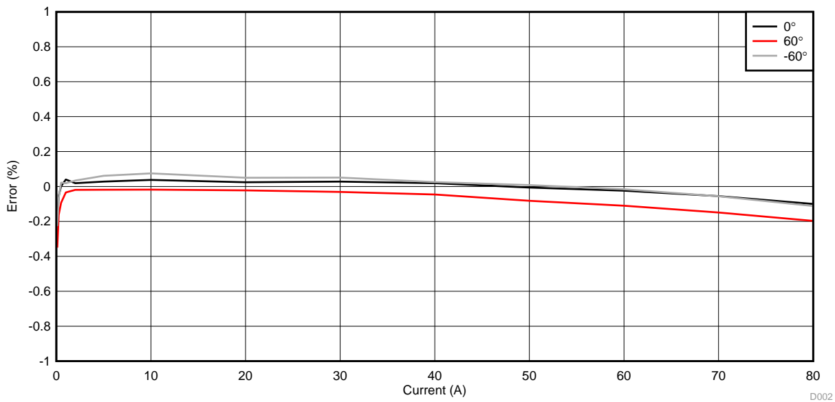
図 38. Cumulative Active Energy % Error Versus Current, 220- \mu\Omega Shunts
