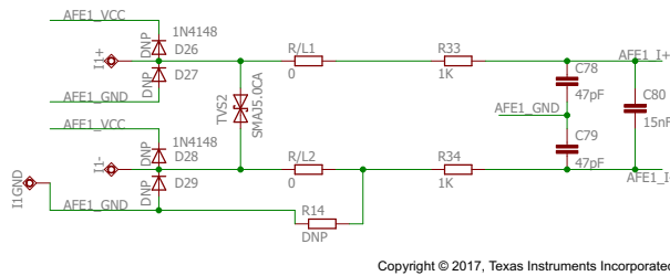
図 7. MSP430i2041 Current Front-End Circuitry
