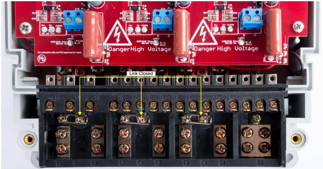
図 20. Top View of EVM With Links Closed
