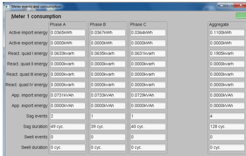
☒ 33. Meter Events and Consumption Window
