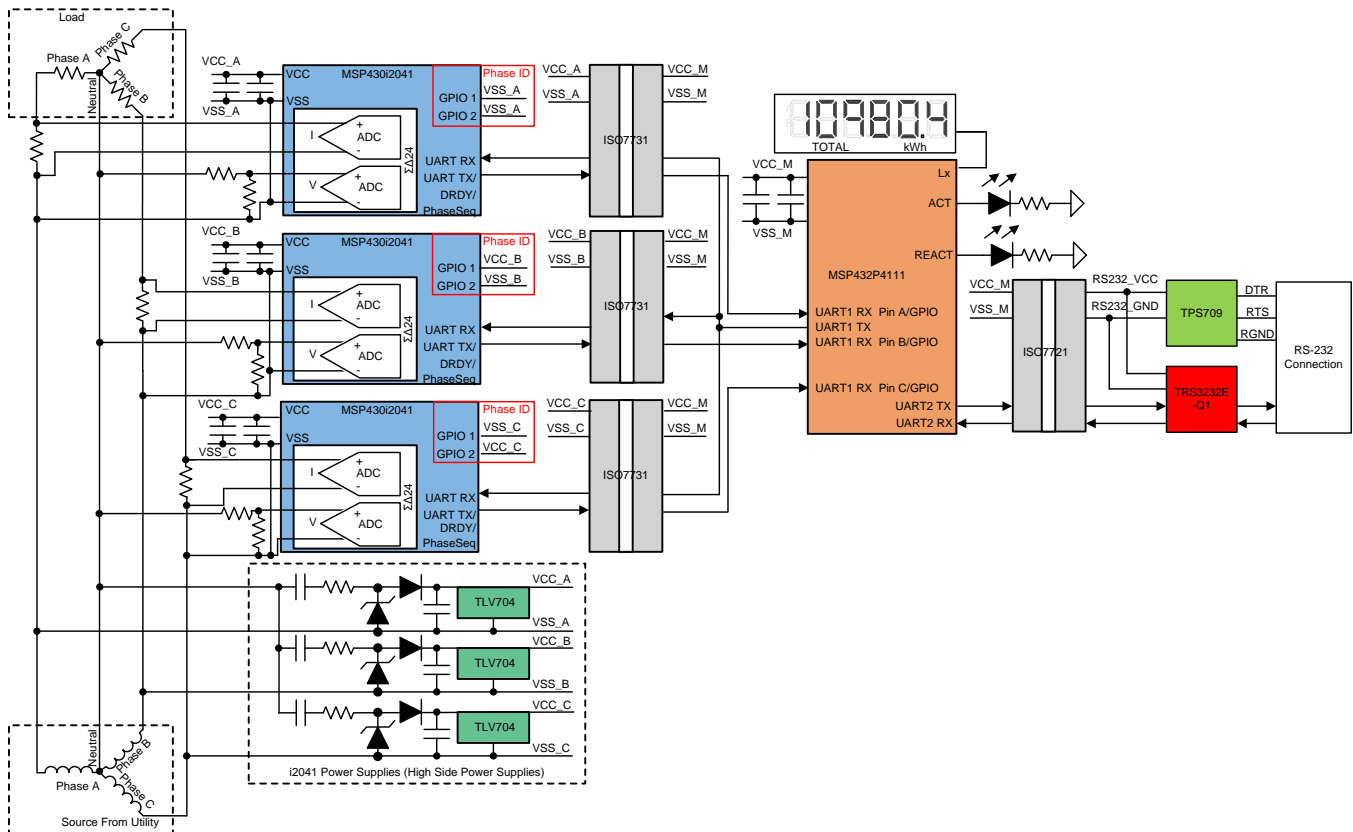
図 2. TIDA-01550 Block Diagram, Two Isolated Channels
