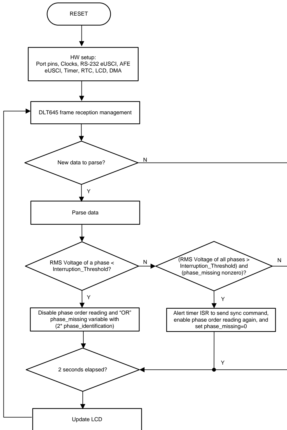
図 12. Peripheral Setup and Idle Tasks
