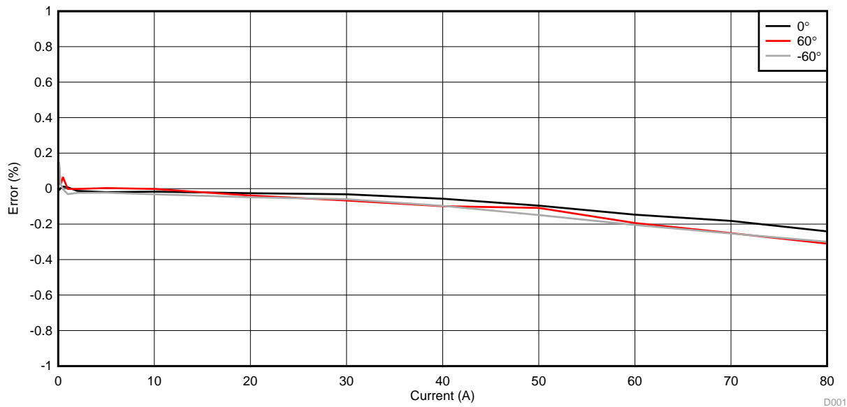
図 37. Cumulative Active Energy % Error Versus Current, 400- \mu\Omega Shunts
