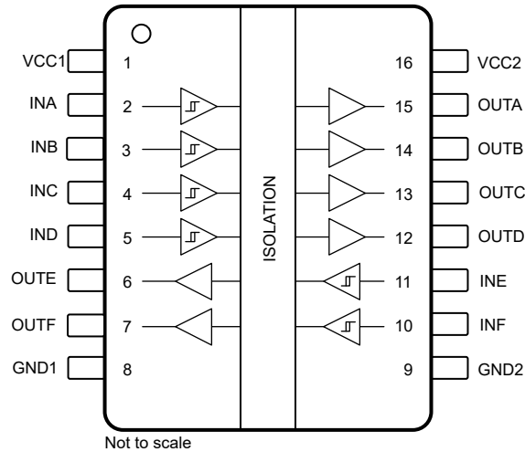
Figure 4-1. Pin Diagram (DW-16 Wide-SOIC Package)
