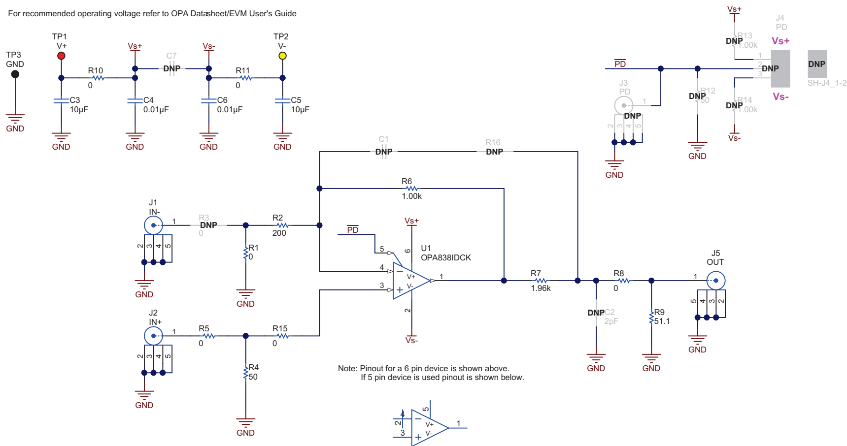
Figure 1. OPA838DCKEVM Schematic
